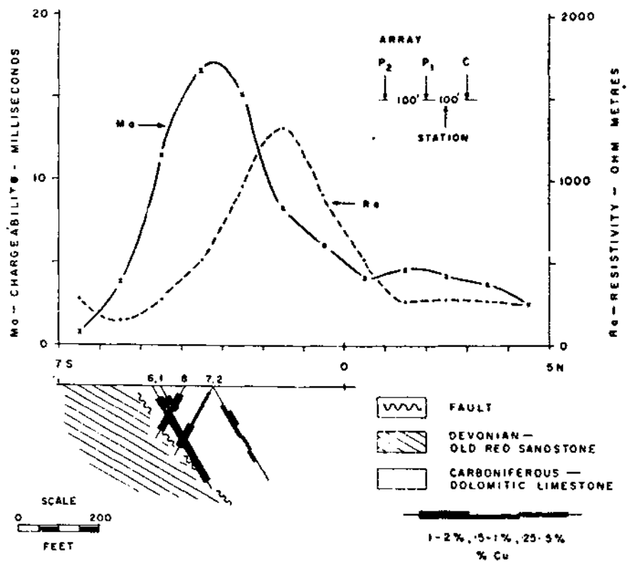
SECTION 200E, FACING WEST 3 ELECTRODE ARRAY - 100'
