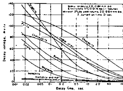
FIGURE 2 Decay Curves for Metallic and Non-metallic Minerals (after Wait, 1959).
