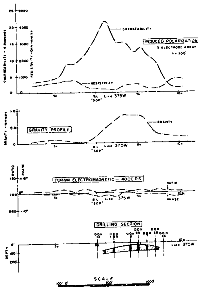
Fig.10. Geophysical and geological section, Pyramid Mines lead-zinc deposit, Northwest Territories, Canada.
