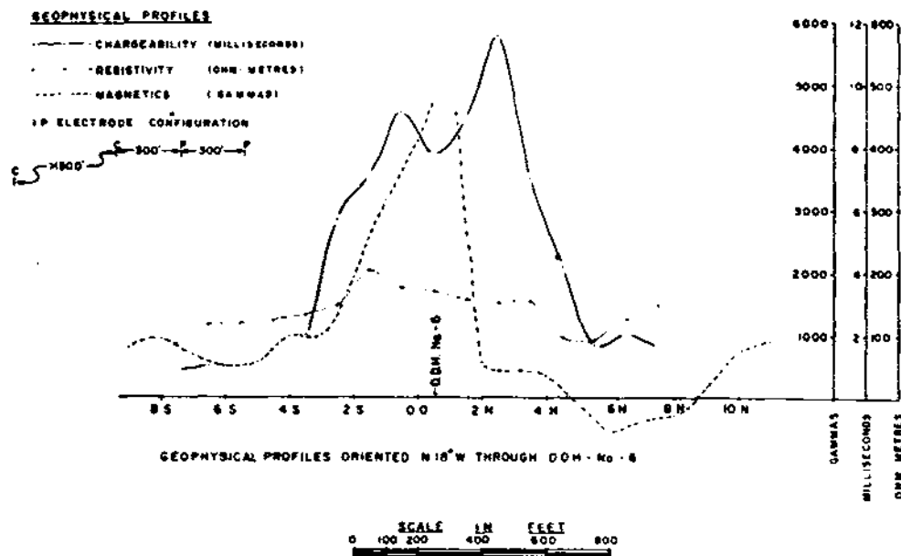
Fig.7. Geophysical section, Craigmont copper deposit, British Columbia, Canada.
