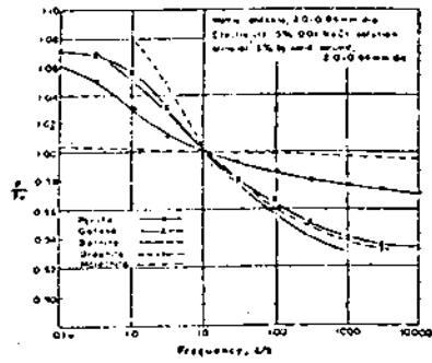
FIGURE 3 Resistivity-frequency Characteristics of Metallic and Non-metallic Minerals (after Wait, 1959).
