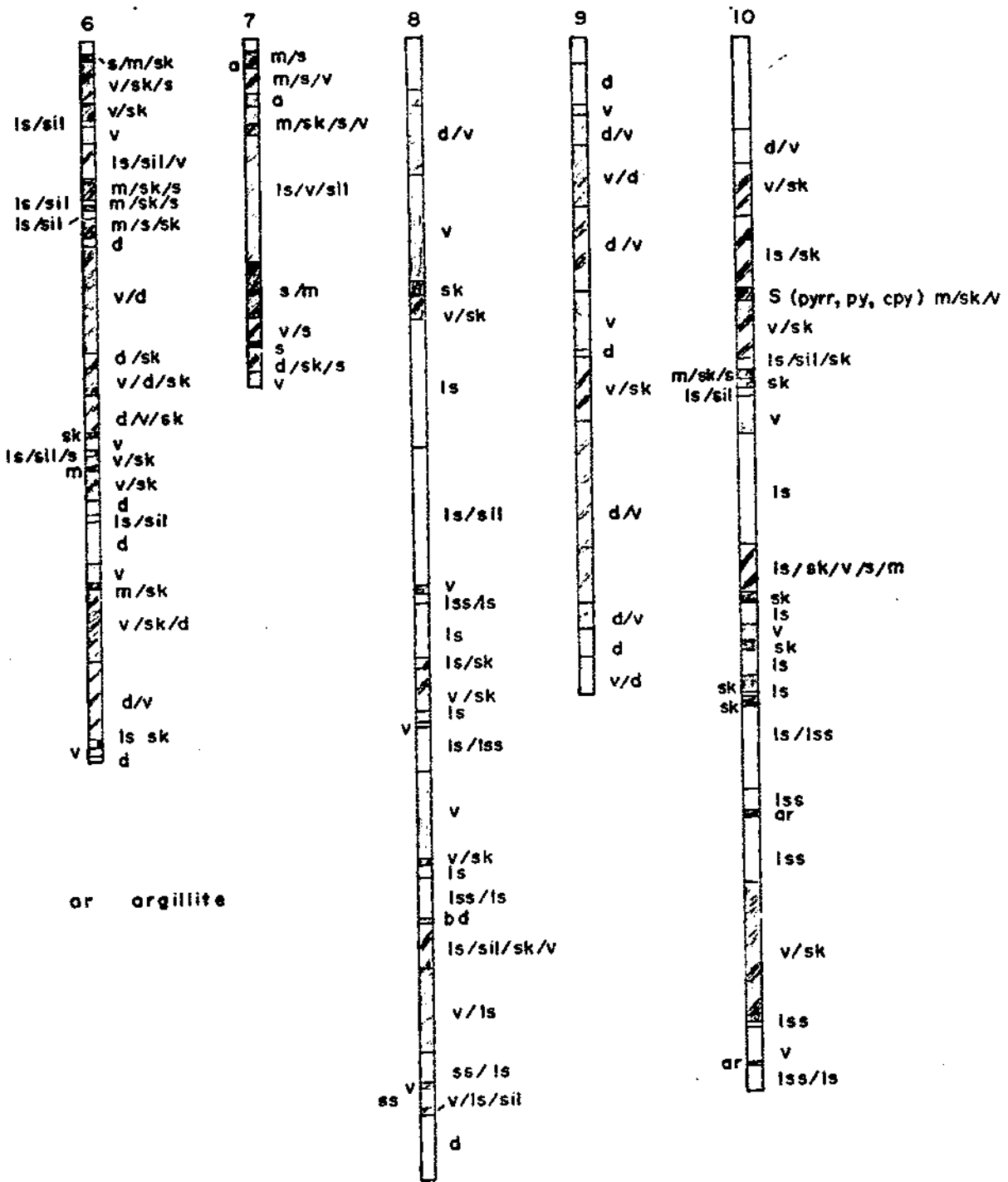
REAKO 'NW' ZONE D.D.HOLE LOGS SCALE : 1" = 50'
