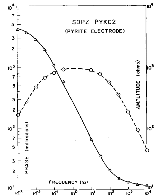
FIG. 16. Amplitude and phase angle spectra obtained by passing current through two pyrite electrodes separated by 5 mm of 0.1 N NaCl solution. The area of each electrode was approximately 4 cm 2 and the electrode surfaces were polished to 20 microns. A 5600-Ω resistor was placed in parallel with the two electrodes.
