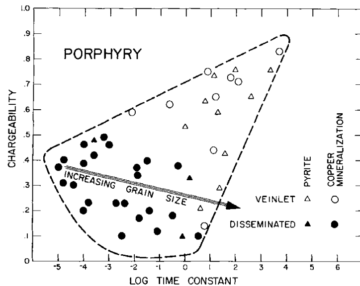
FIG. 14. Data from porphyry deposits plotted in chargeability-time constant space. There is a grouping of veinlet mineralization (open symbols) versus discretely disseminated mineralization (closed symbols) but there is no distinct grouping of pyrite mineralization (triangles) versus copper mineralization (circles). Superimposed on the plot is the arrow from Figure 6 which indicates the trend due to increasing grain size in artificial rocks.
