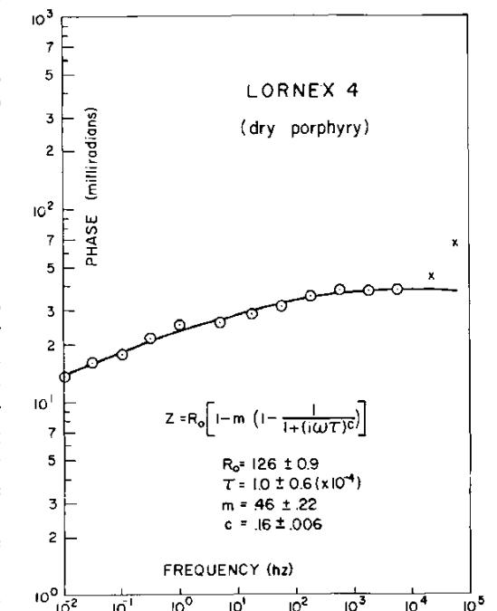
FIG. 8. Phase angle spectra from the Lornex porphyry copper deposit in Highland Valley region of British Columbia. Dipole-dipole array: n = 1 , x = 1 m. The circles represent the observed data, the solid line represents the best-fitting theoretical curve, and the crosses represent possibly noisy data which were not used in the inversion.
