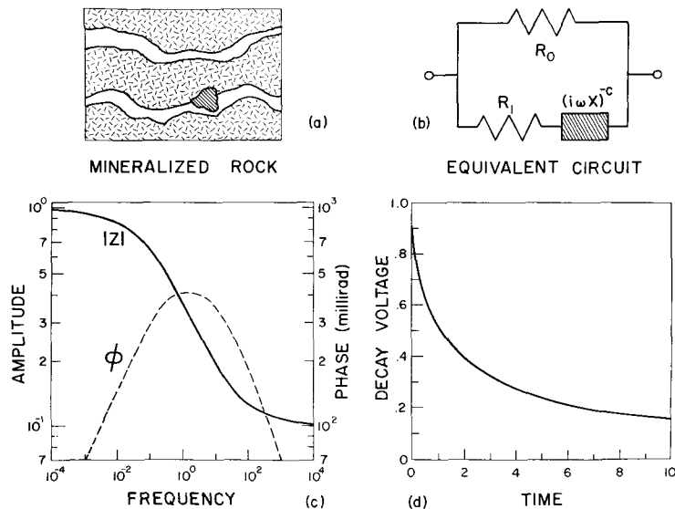
FIG. 1. (a) A small section of a mineralized rock which has both blocked and unblocked pore passages. (b) An equivalent circuit for the mineralized rock. (c) Typical frequency domain response for the equivalent circuit. (d) Time domain response corresponding to the frequency domain response plotted in (c).
