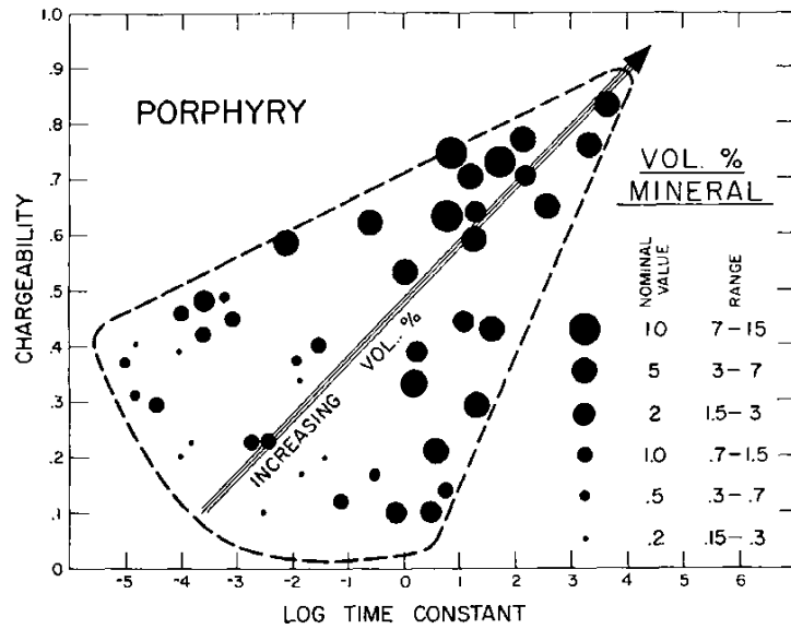
FIG. 13. Data from porphyry deposits plotted in chargeability-time constant space. The larger dots indicate high sulfide concentration. Superimposed on the plot is the arrow from Figure 6 which indicates the trend due to increasing volume percent sulfides in artificial rocks.
