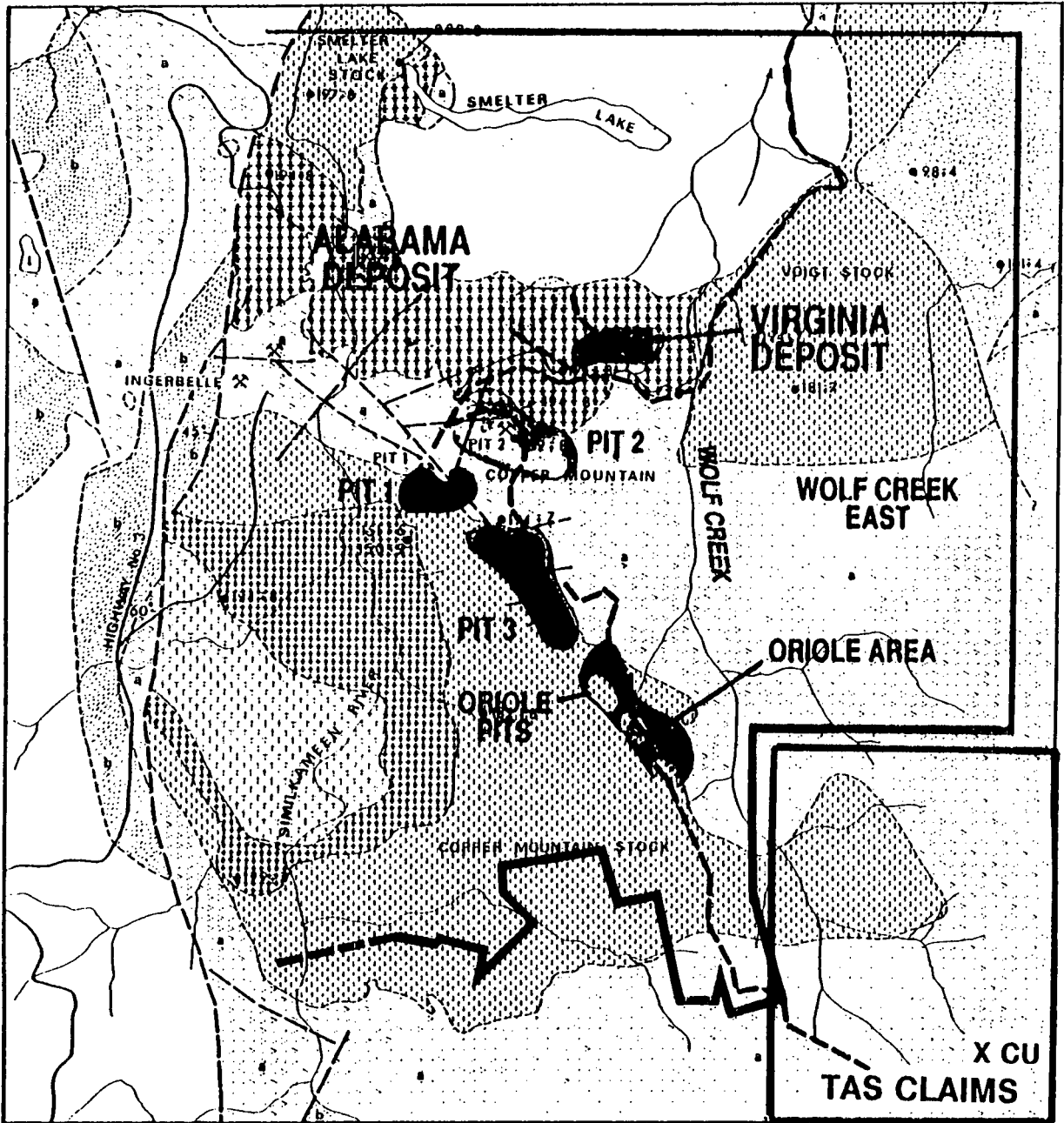
GENERALIZED GEOLOGY OF THE COPPER MOUNTAIN AREA
