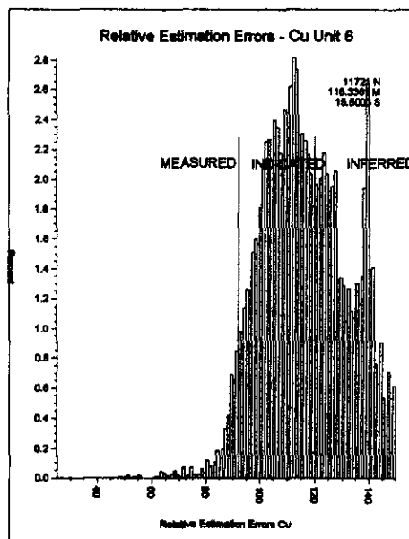
Figure 18: Histograms for Relative Estimation Errors in Cu for Units 4, 1-3 and 6
