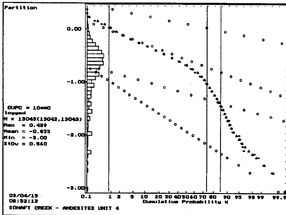
Figure 10: Lognormal Cumulative Frequency Plot for Cu in Andesites
