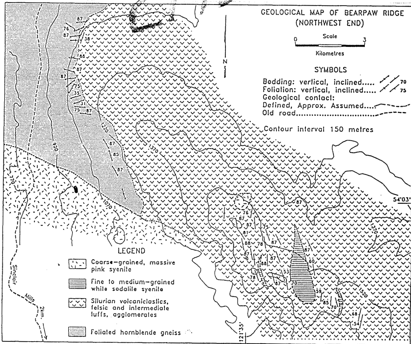
FIGURE 2 GEOLOGICAL MAP OF BEARPAW RIDGE
