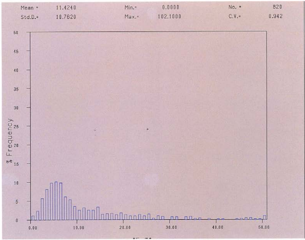
Figure 11: Histogram and Basic Statistics of all Fe% samples.
