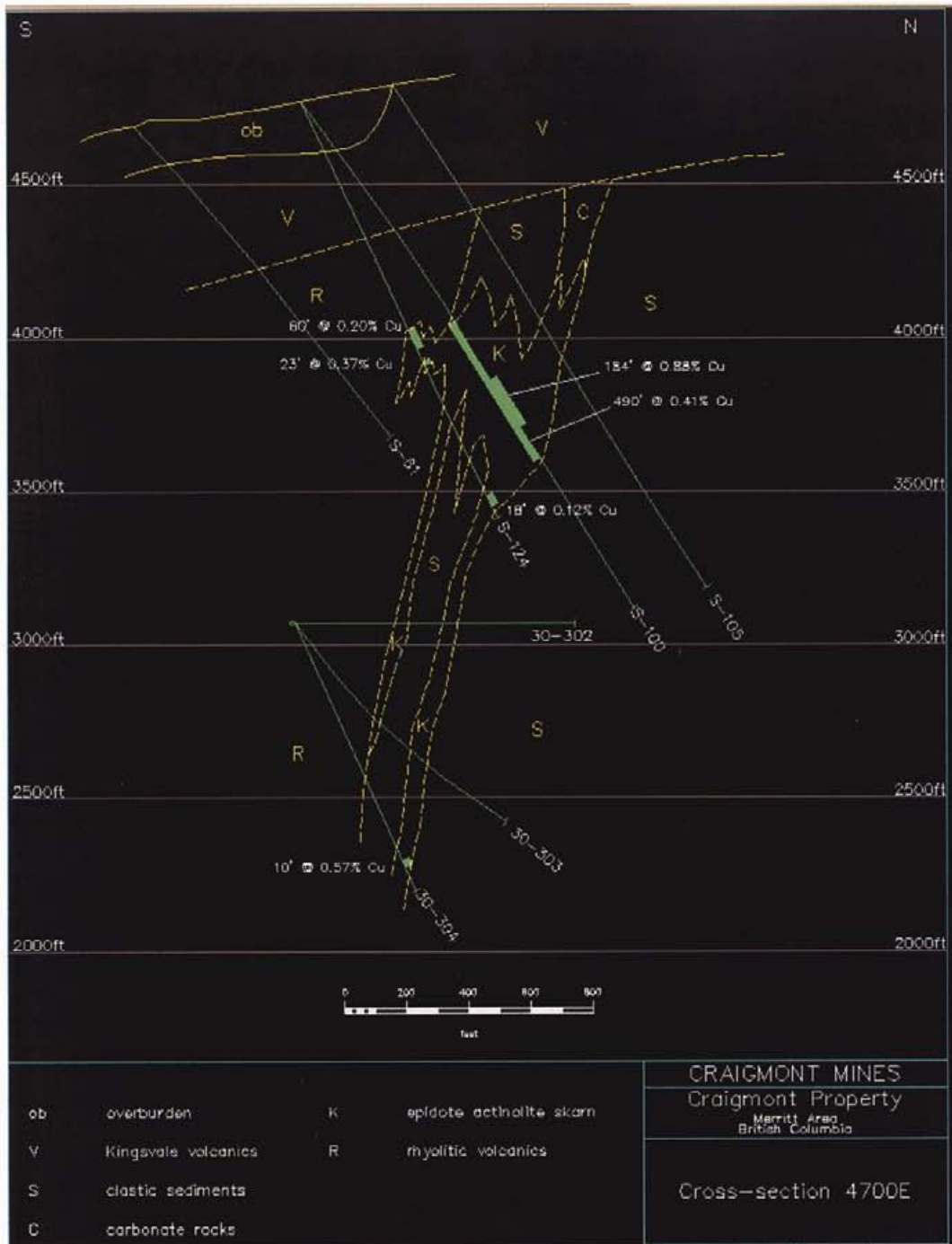
Figure 35: 4700E Cross-section considered to be the primary target for mineralization within the Embayment Block.
