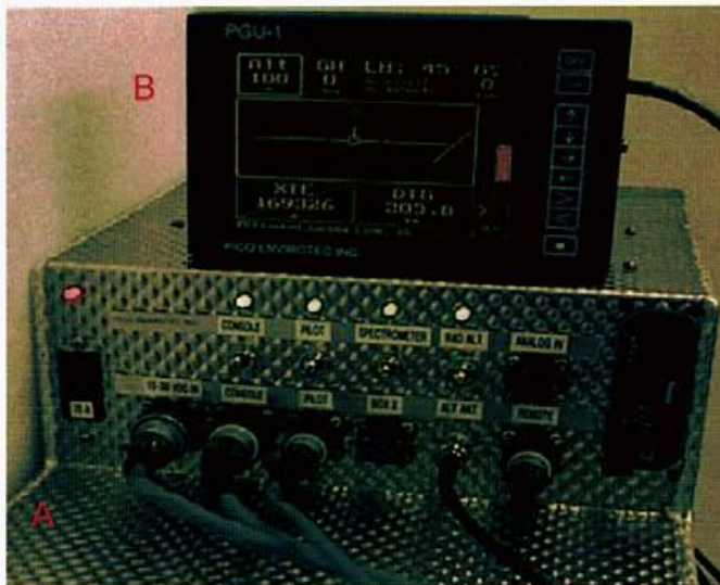
Figure 7. Aeroquest AGRS system. A. AGRS Sensor (Crystal Pack), B. Data acquisition computer.
