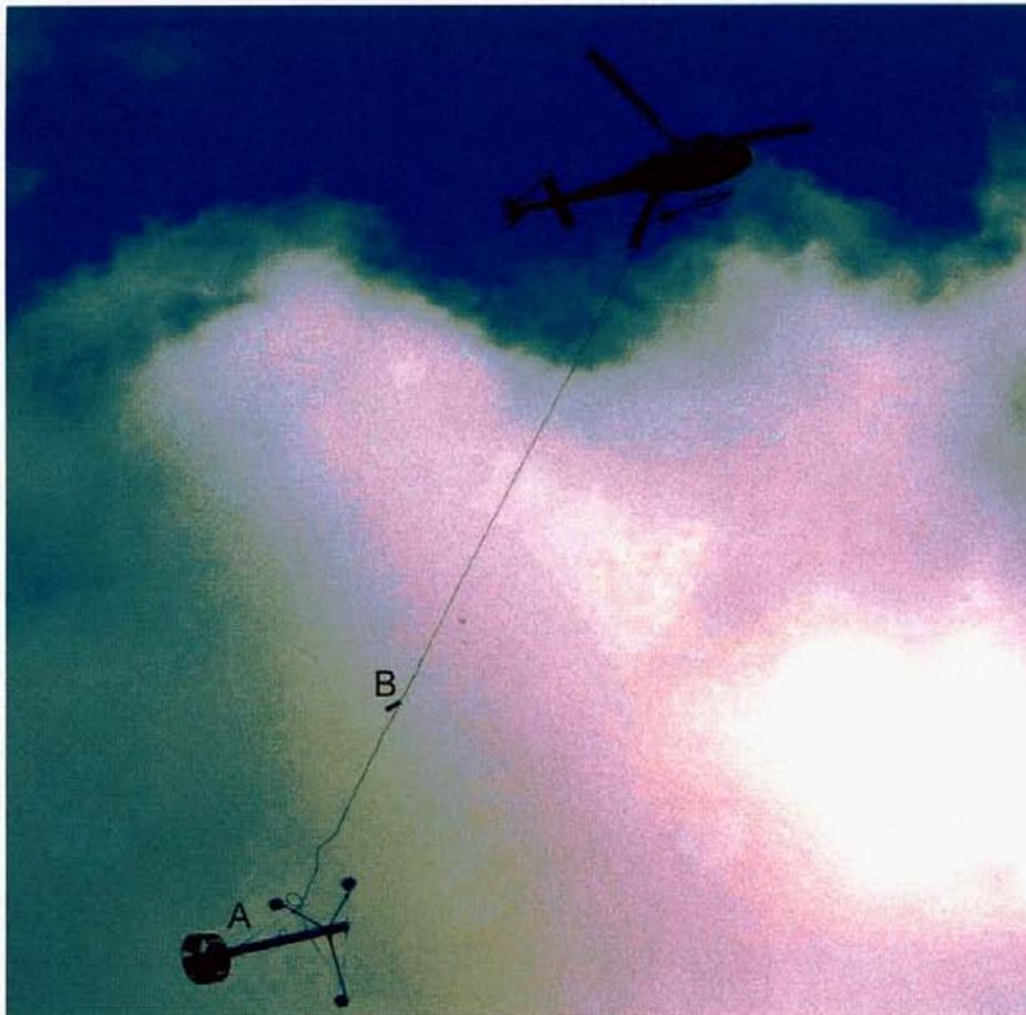
Figure 6. The gradiometer bird (A), and GPS antenna (B). The AGRS system is located in the helicopter cabin.
