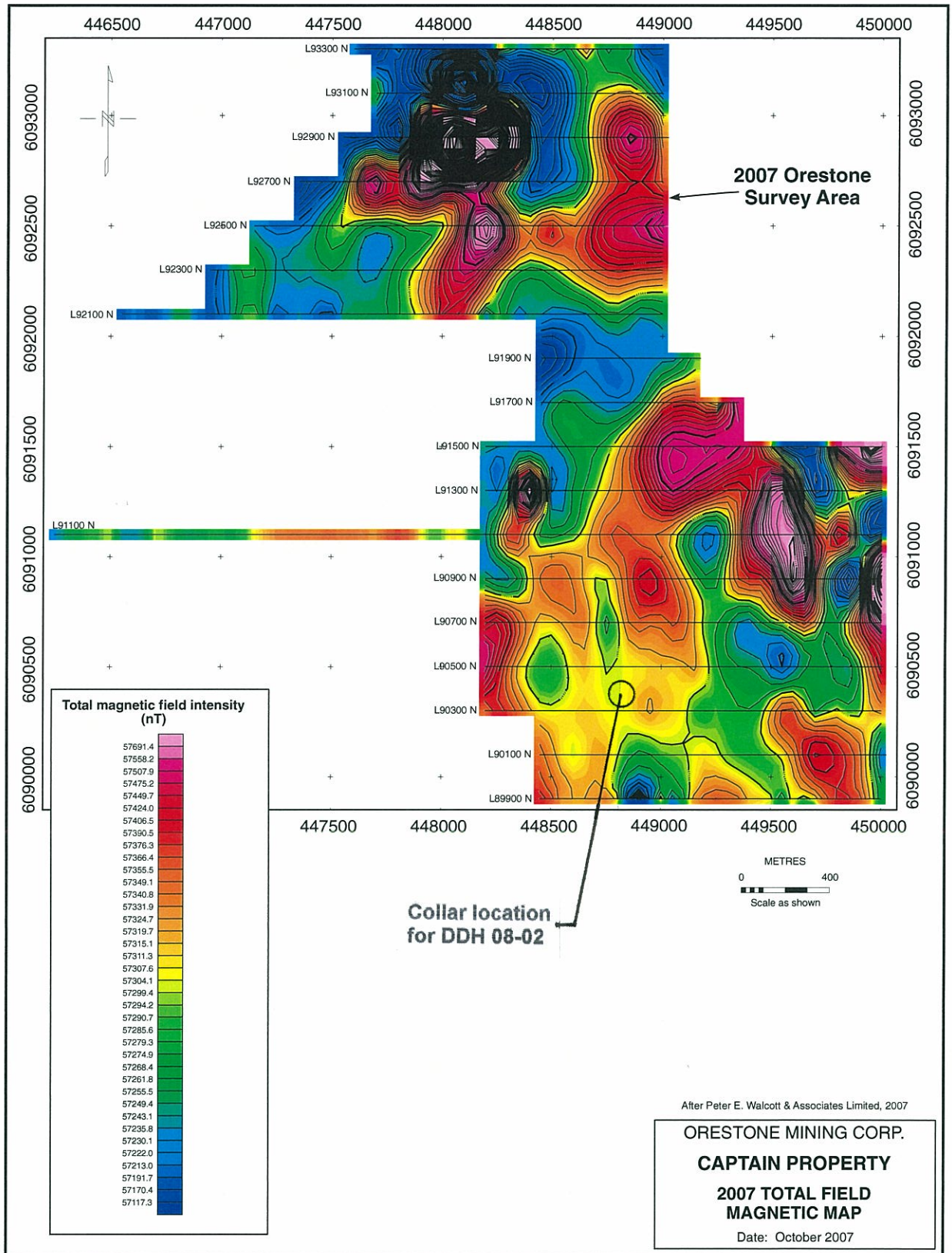
Figure 5 - 2007 Total Field Magnetic Map, Captain Property (CP)
