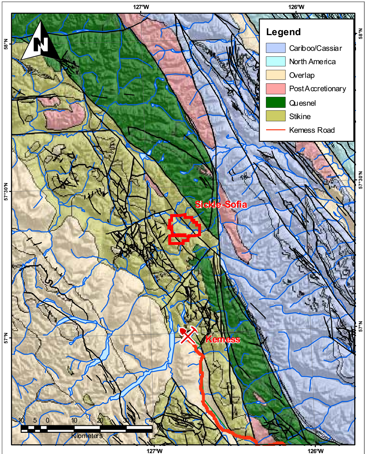
Figure 4 Regional geological setting
