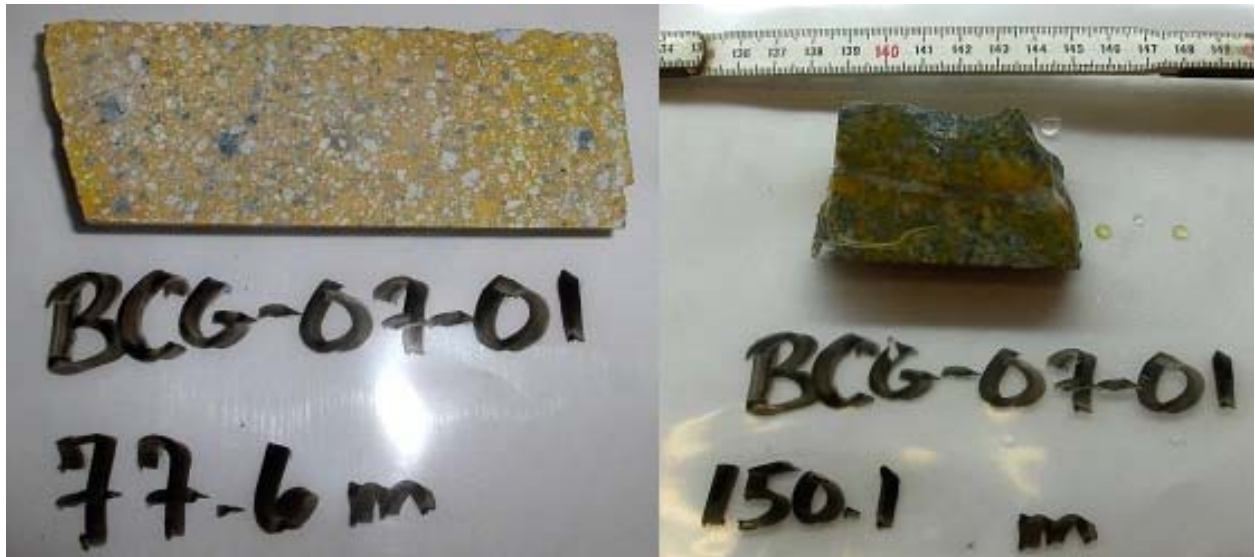
Figure 5 Potassic alteration of intrusive monzonite at 77.6m depth and along quartz vein selvage at 150.1m.
