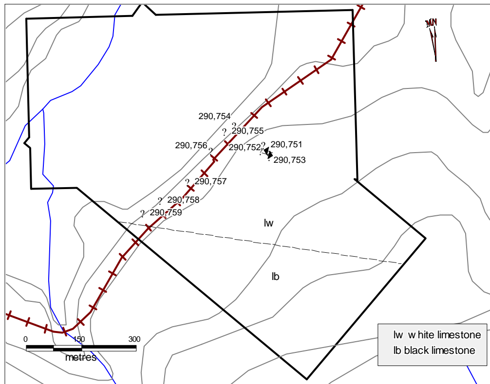
UTM NAD 83 Zone 9 NORTH ISLAND CARBONATE PROJECT Beaver Property Sample Locations Figure 6a
