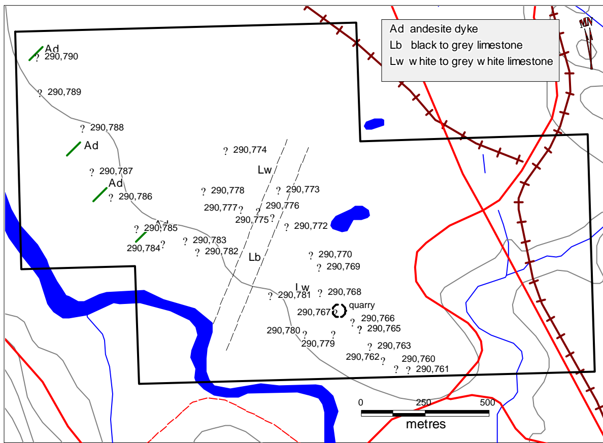
NORTH ISLAND CARBONATE PROJECT Dump Property Sample Locations
