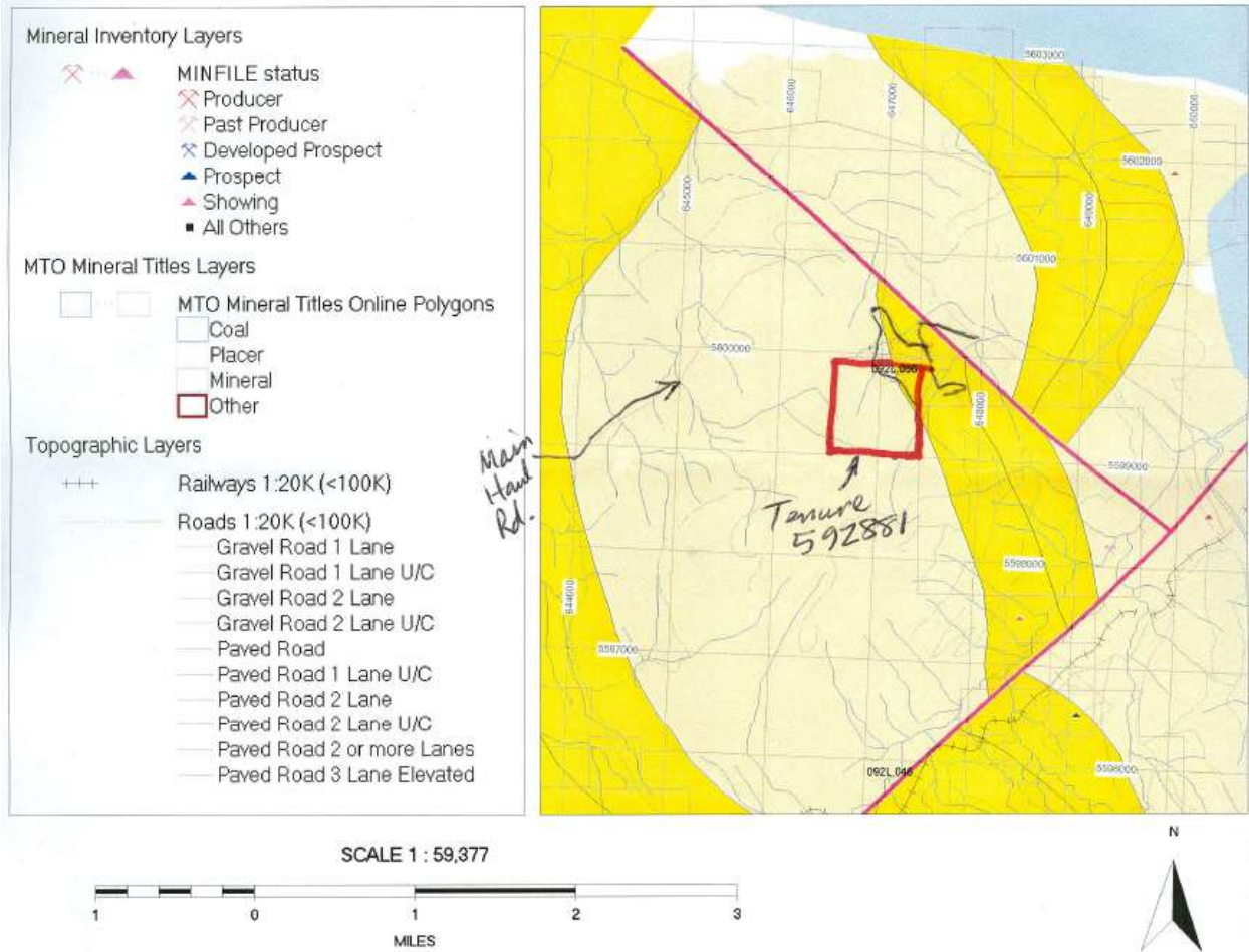
Figure 5a Detail Regional Geology
