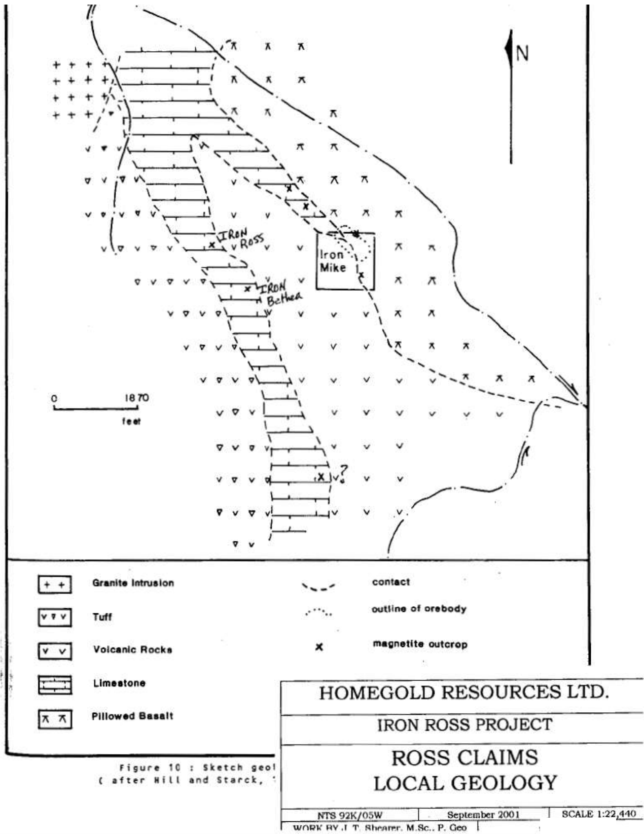
Figure 7 Local Geology (Generalized)
