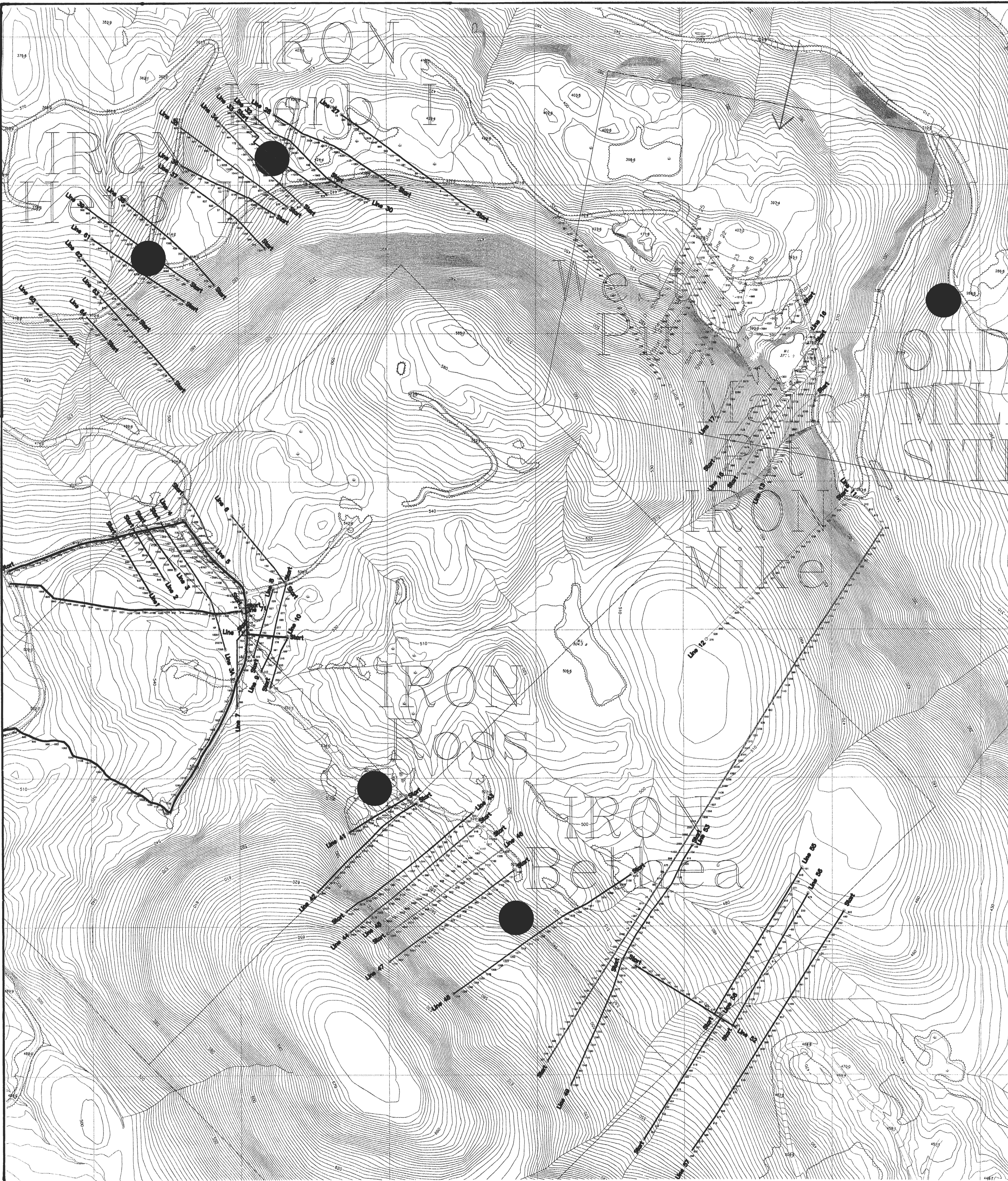
FIGURE II IRON ROSS PROJECT LOCATION of Magnetometer Lines
