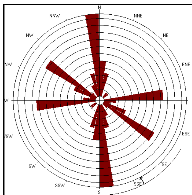
Figure 6. Rose Diagram from lineaments of Tenure 589951 (Figure 5)
