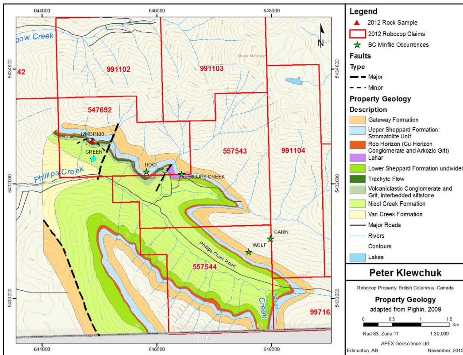
Figure 8 Property Geology
