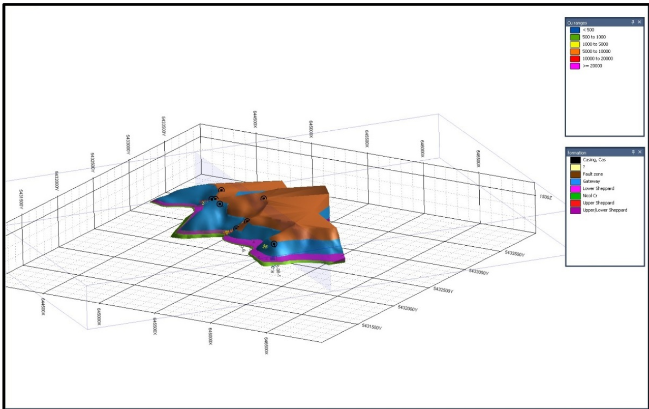
Figure 9 3D Micromine model of drilling (top) and geology (bottom) at the Robocop Property.
