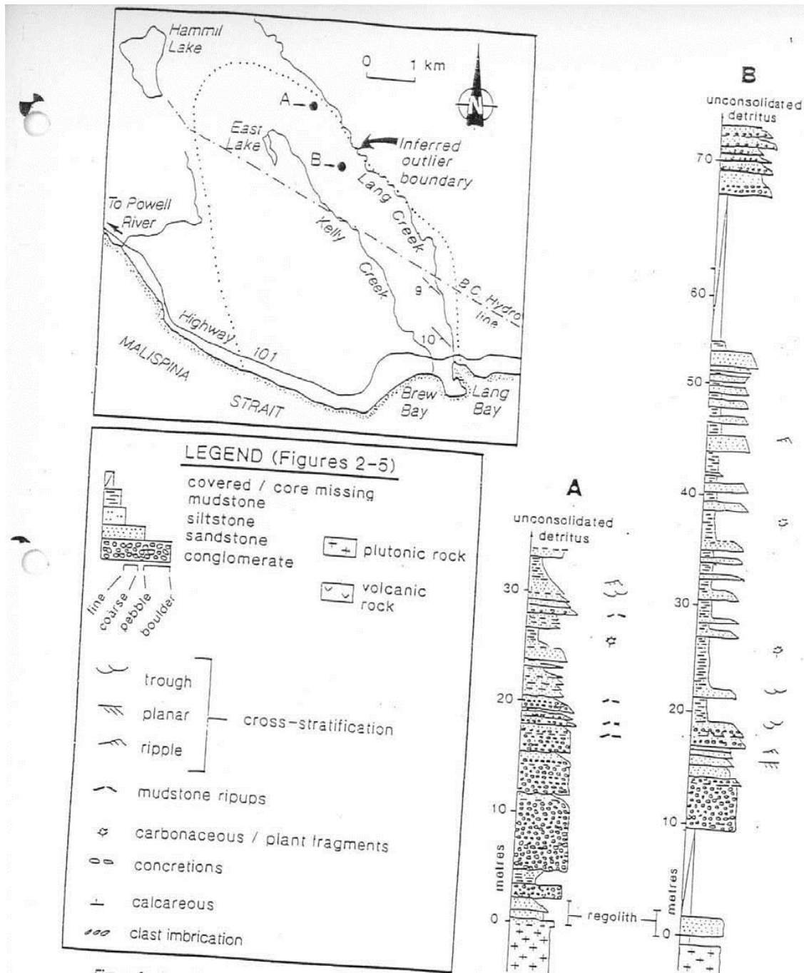
Figure 2. Lang Bay outlier with logs from two drillholes. Outlier boundary is modified from White (1986). (after Mustard + Rowsee).
