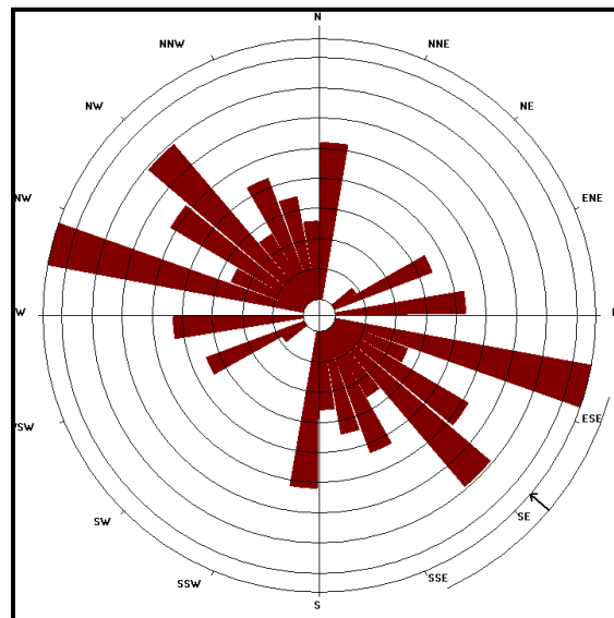
Figure 6. Rose Diagram from lineaments of Figure 5
