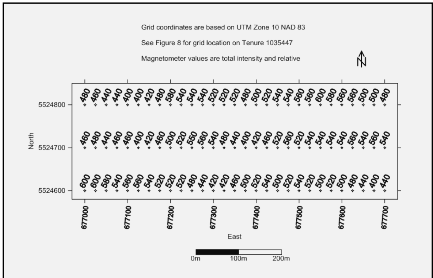
Figure 9 .Magnetometer Survey Grid & Raw Data (Base from MapPlace)
