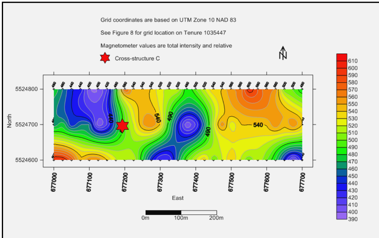
Figure 11. Magnetometer Survey Coloured Contour Map
