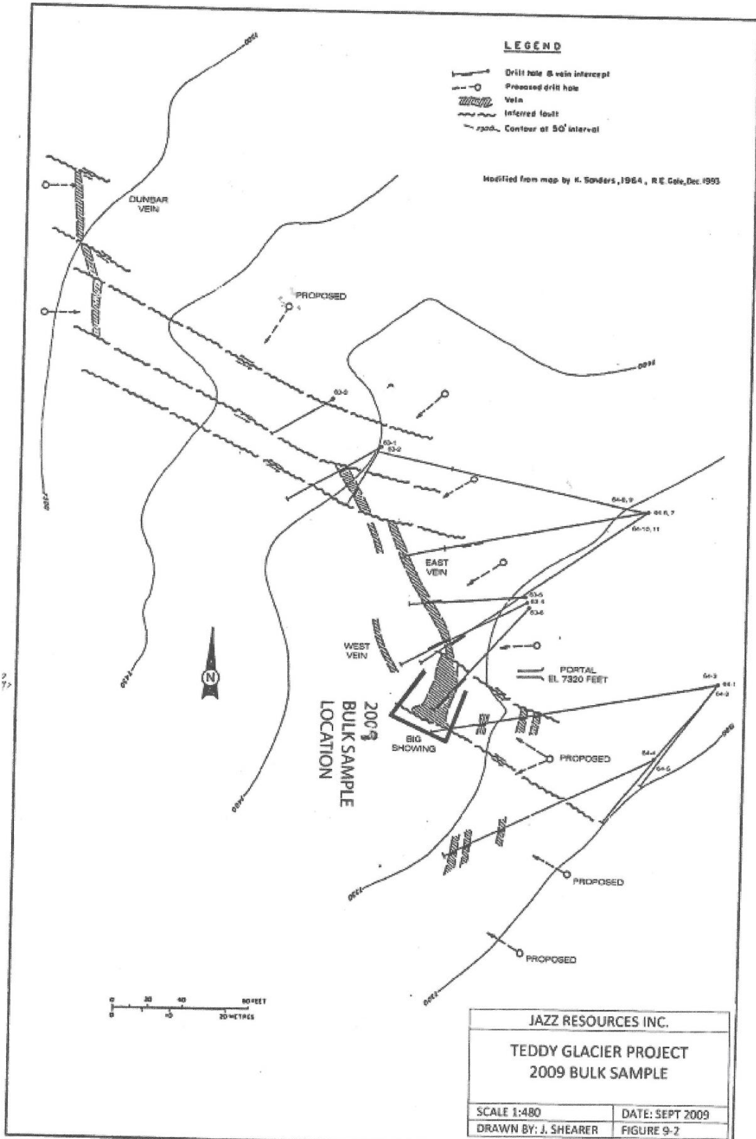
Figure 5 Bulk Sample
