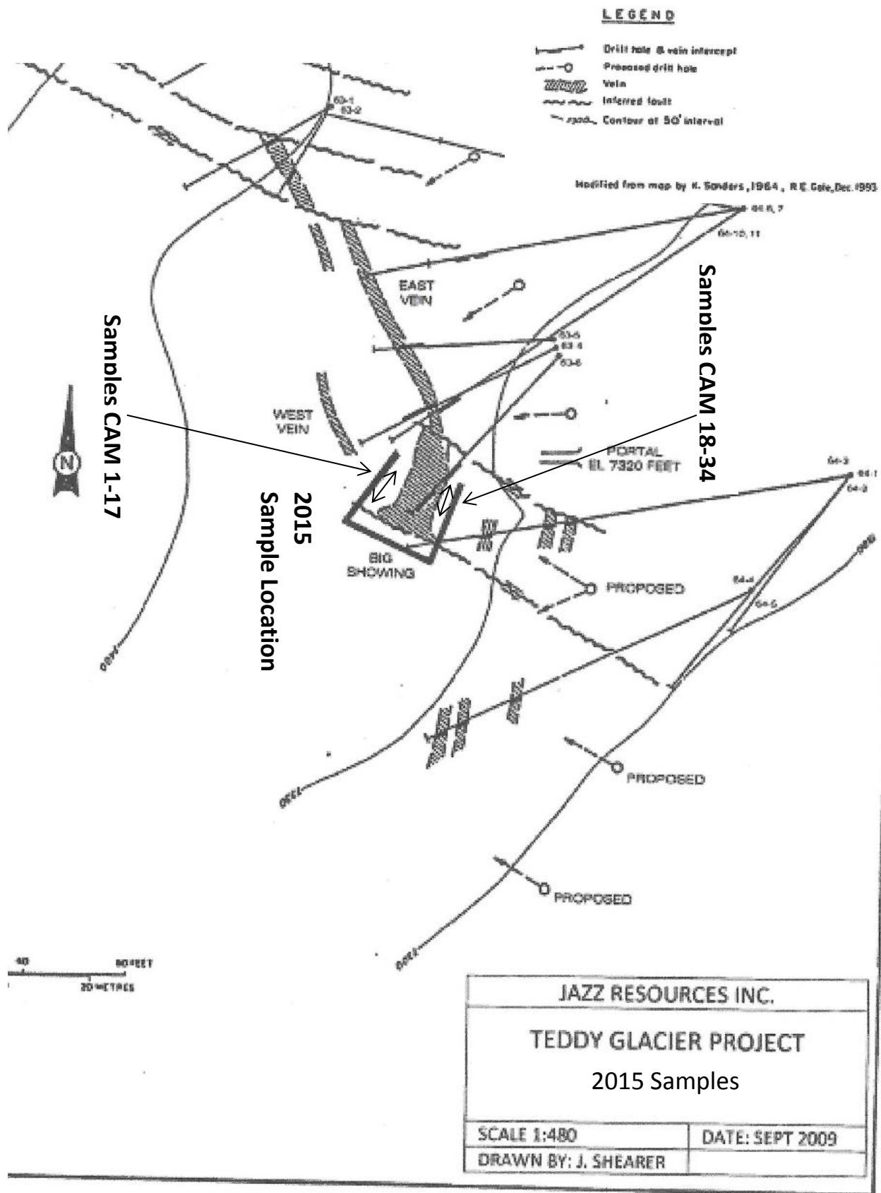
Figure 7 Sample Locations
