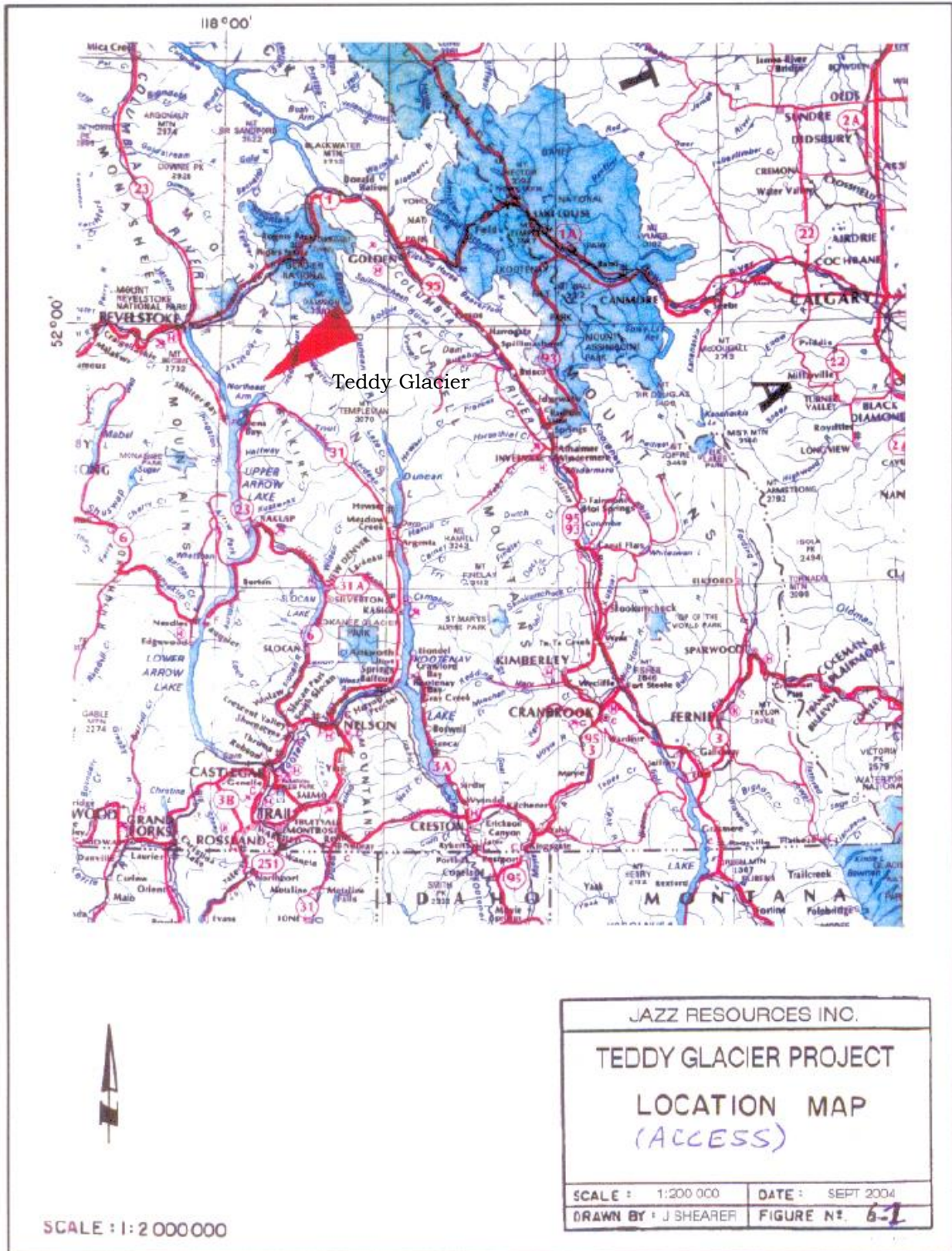
Figure 2 Access Map
