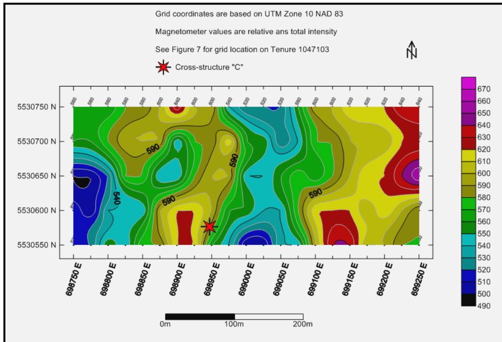
Figure 11. Magnetometer Survey Data Coloured Contour Map
