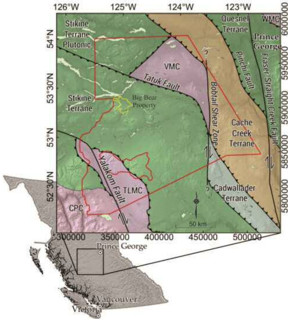
Figure 3. Regional Geology (Angen et al. , 2016).
