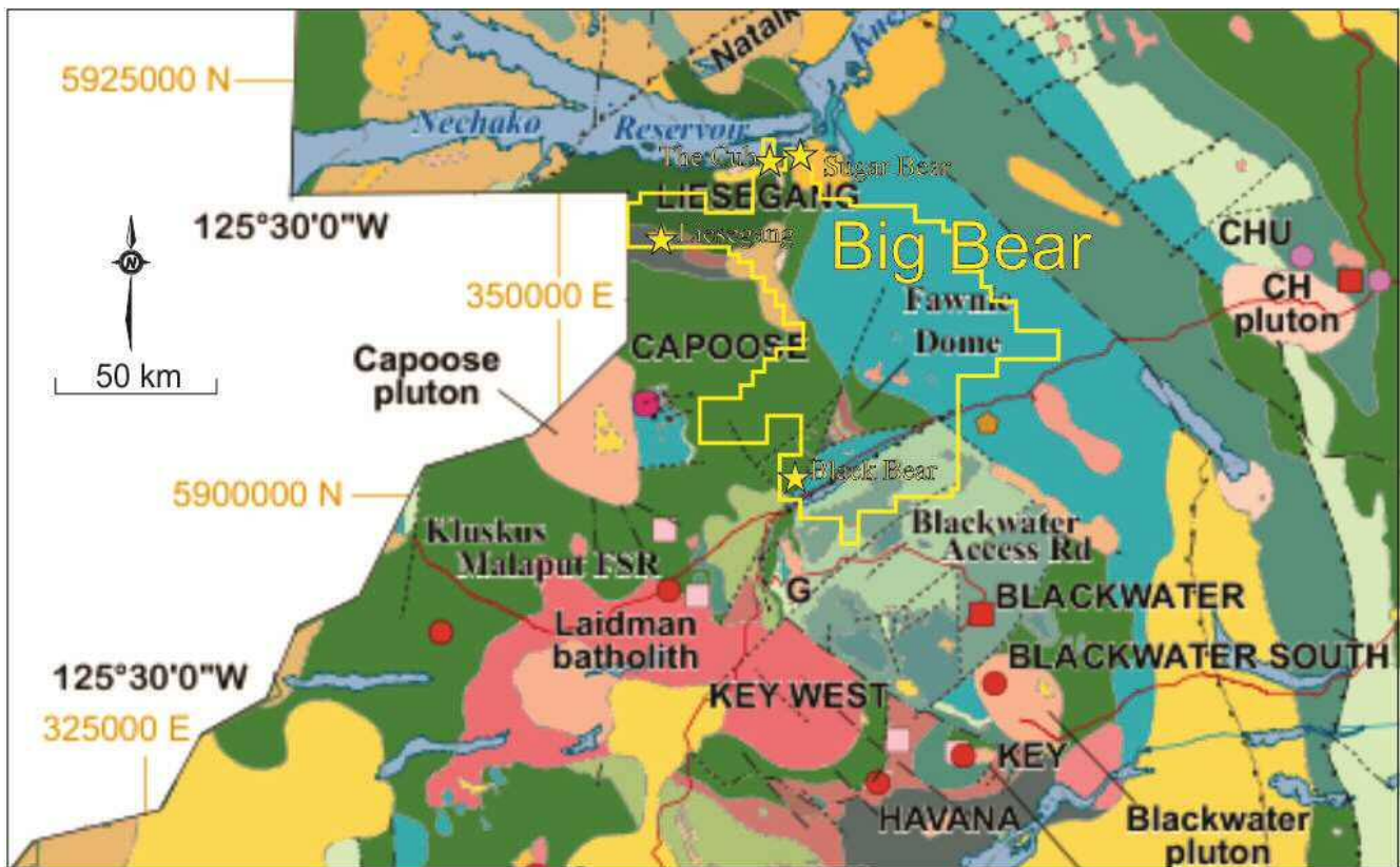
Figure 4. Property Geology (after Angen et al. , 2016)
