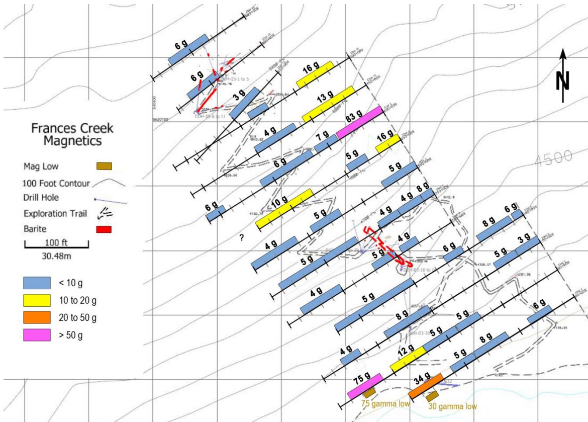
FIGURE 9.2 Magnetic Survey - Frances Creek Property
