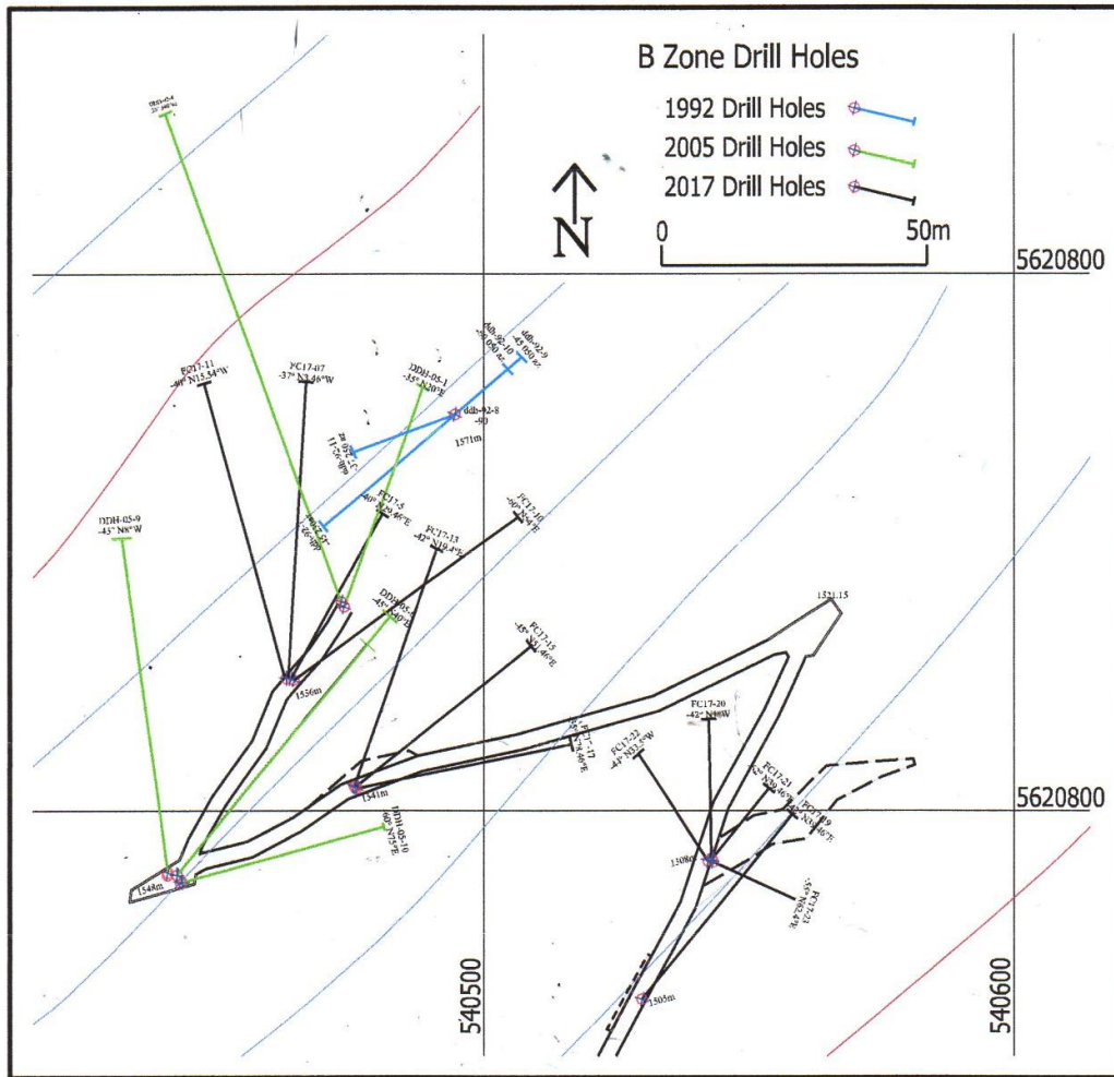
Figure 10.2 – Drill Hole Map – Zone B
