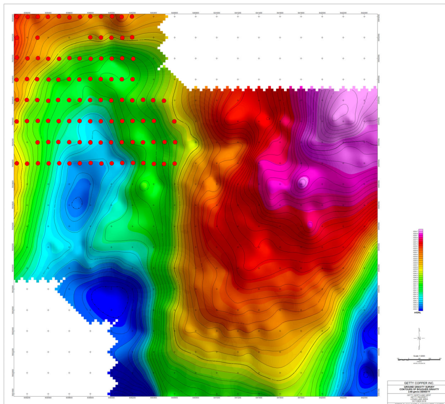
Contours of Bouguer Gravity 2.65 gm/cc - 2018 Stations in Red
