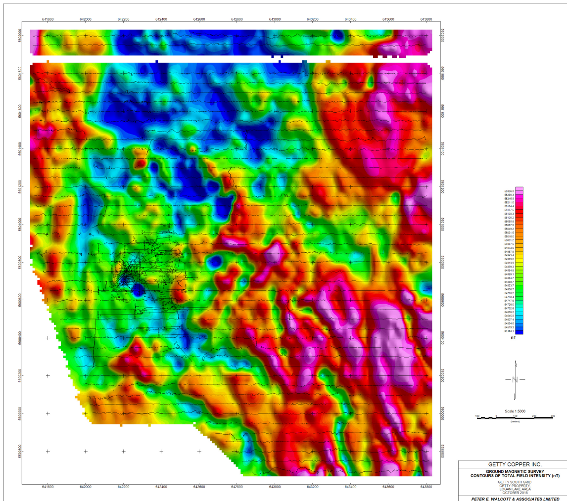
Contours of Total Field Intensity (nT) Getty South
