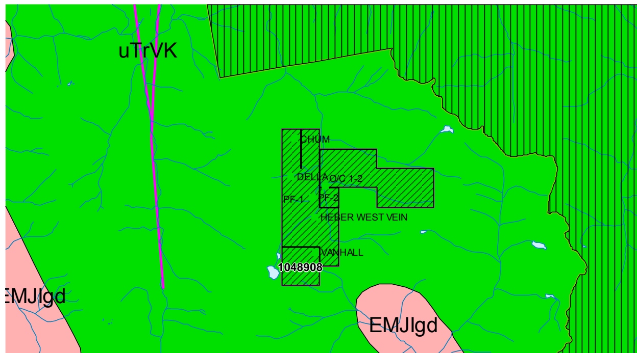
Figure 10: Property Geology.
