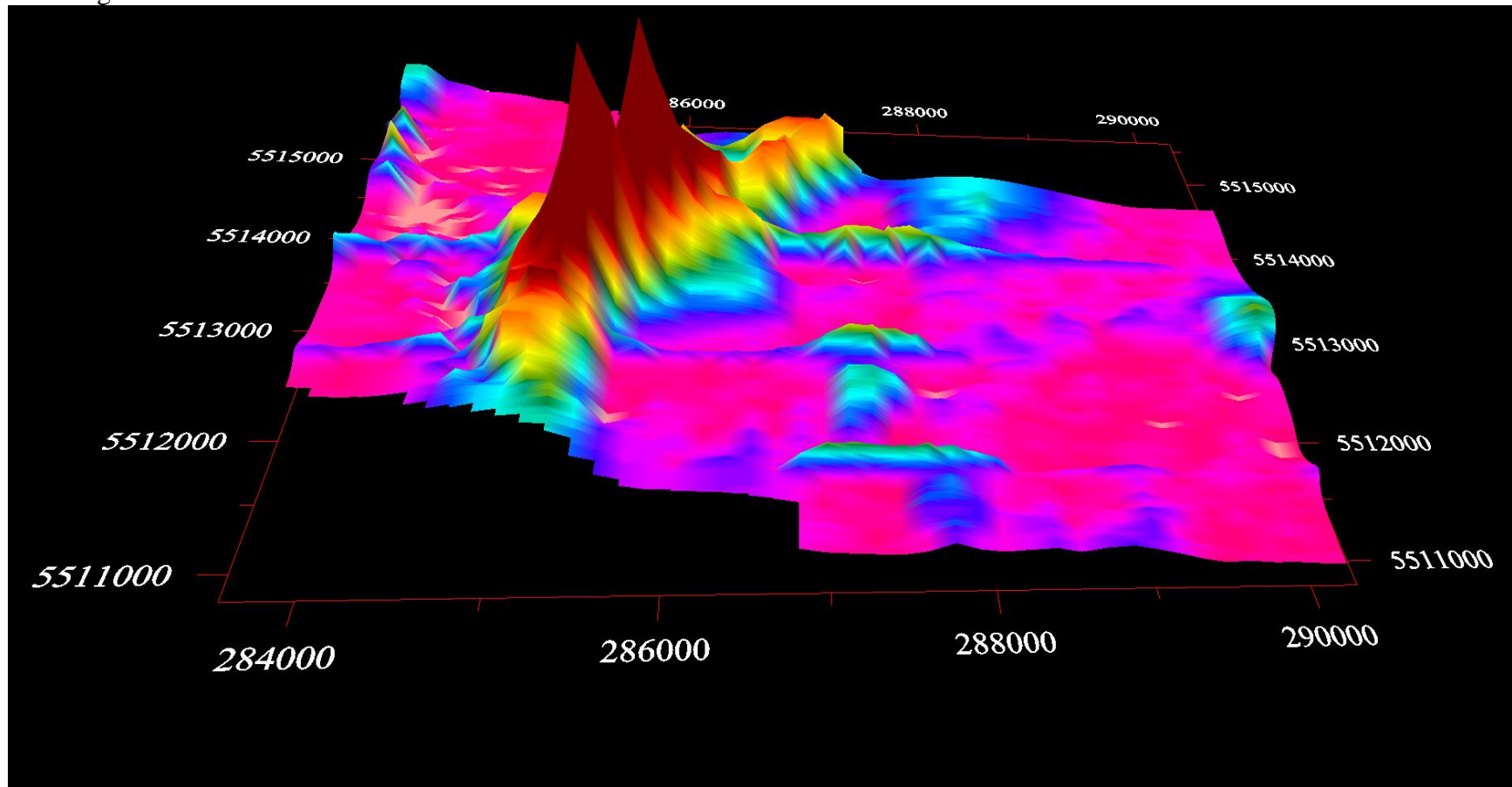
3D view of EM channel 2 amplitude
