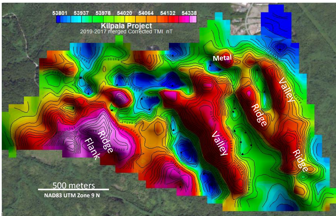
Figure 6. The sun shaded base corrected 2019-2017 merged TMI image on Landsat. The raw data range is 7507 nT, the 40 m cell gridded range is 1572 nT. There is a broad correlation on the east half of the image between magnetic responses and topography, as labeled.
