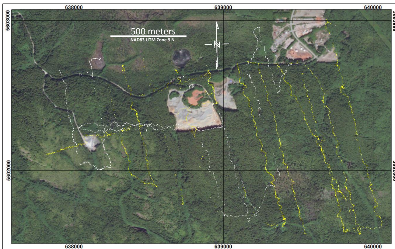
Figure 1. Kilpala 2019 ground magnetic survey lines the white traverses, with about 7 line km surveyed. The yellow lines are the 2017-2018 survey traverses, covering about 15 km, for a merged total 22 km.
