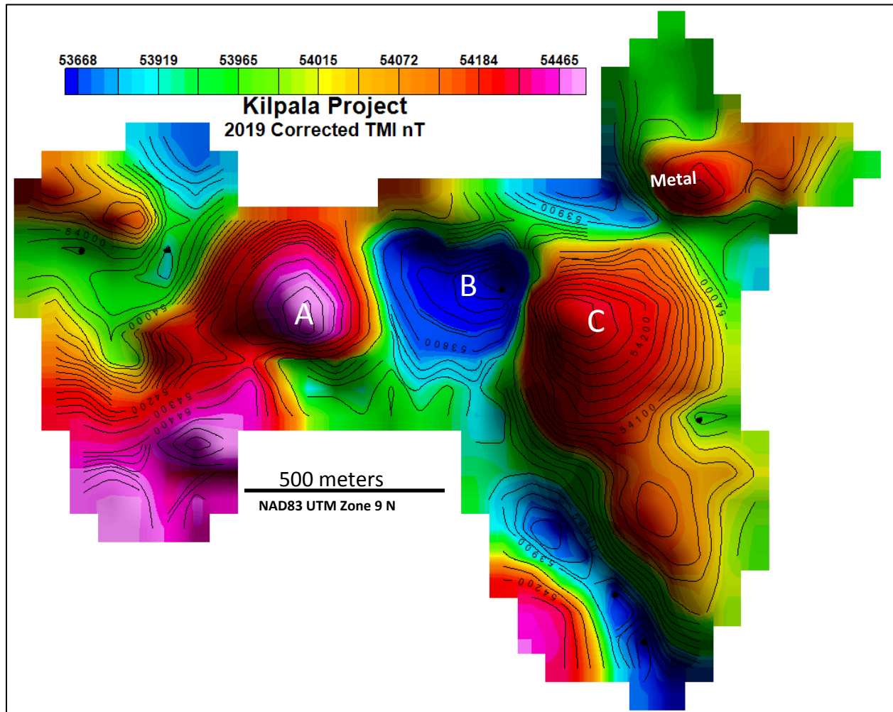
Figure 4. The sun shaded base corrected 2019 TMI image. The raw data range is 7507 nT, the 60 m cell gridded range is 1729 nT. Metal culture is seen on the NE. The prominent signatures at sites A, B and C are suspect and look like gridding artifacts for a lack of survey line coverage across them, and that are also shown in Figure 5.
