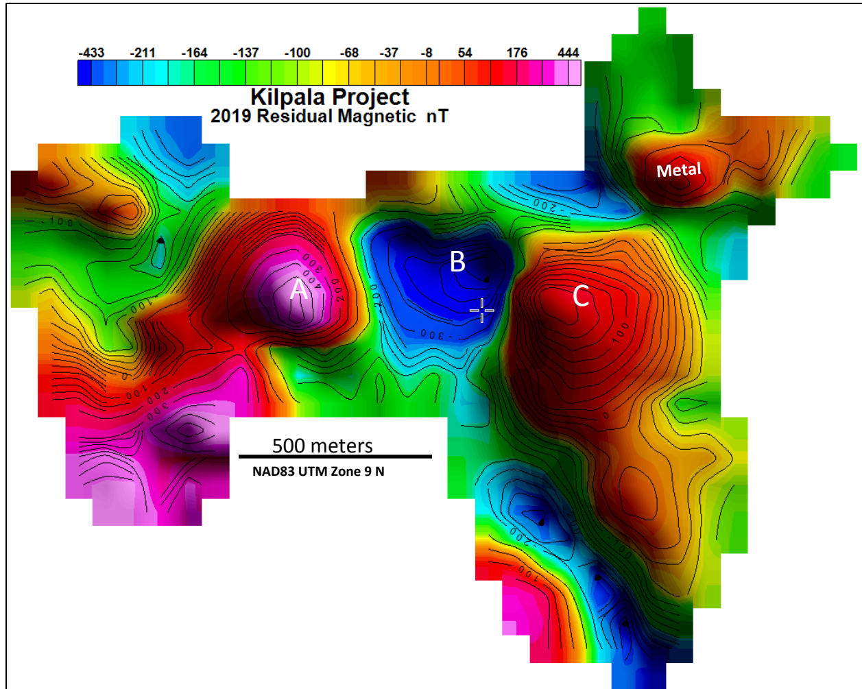
Figure 5. The sun shaded IGRF corrected residual magnetic image. The raw data range is 7506 nT, the 60 m cell gridded range is 1734 nT. Metal culture is seen on the NE.
