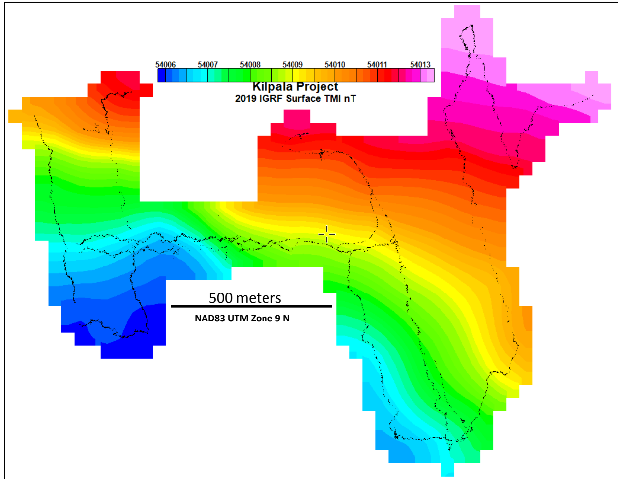
Figure 3. IGRF correction values across the 2019 Kilpala grid, range is 5 nT.
