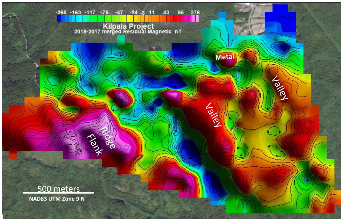
Figure 7. The sun shaded IGRF corrected residual 2019-2017 merged TMI image on Landsat. The raw data range is 7506 nT, the 60 m cell gridded range is 1845 nT. The valley responses remain obvious.
