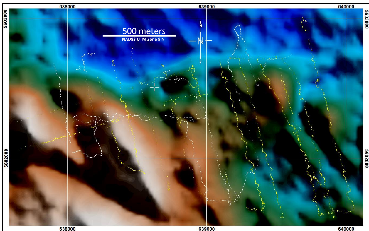
Figure 2. Kilpala area SRTM image with the 2019 magnetic survey sample lines the white traces, 2017-2018 survey lines the yellow traces. There is 138 metres of topographic relief in the survey area.
