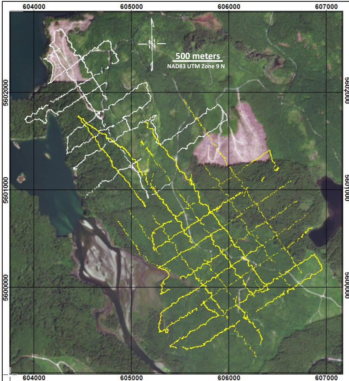
Figure 1. The Varney Bay 2019 ground magnetic survey sample lines the white traverses, with about 13 line km surveyed. The yellow lines are the 2017-2018 survey traverses, covering about 31 km, for a total 44 km.
