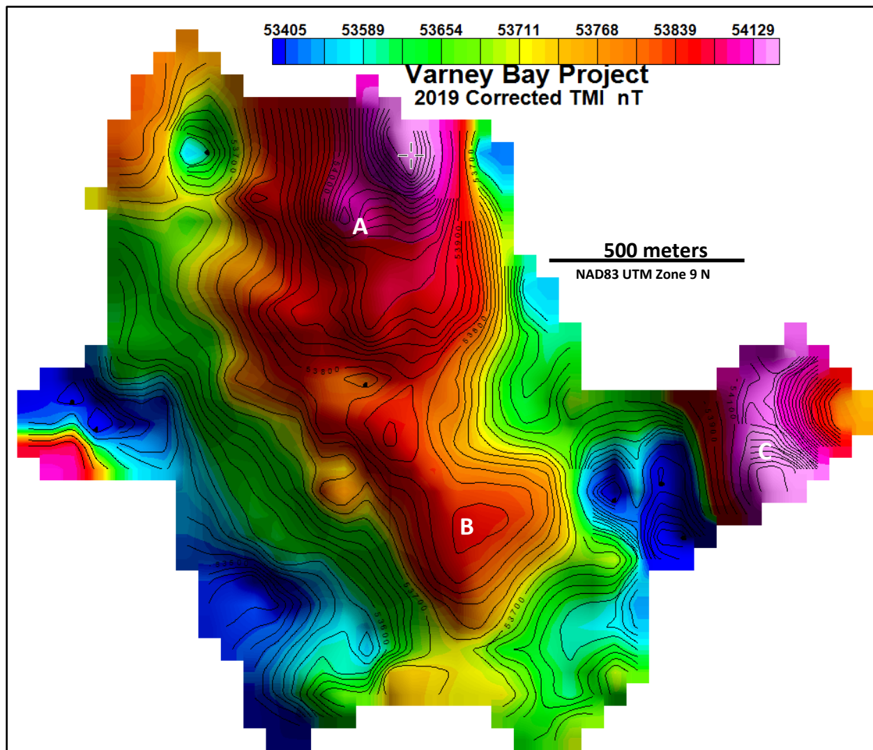
Figure 4. The sun shaded base corrected 2019 TMI image. The raw data range is 3595 nT, the 60 m cell gridded range is 1521 nT.
