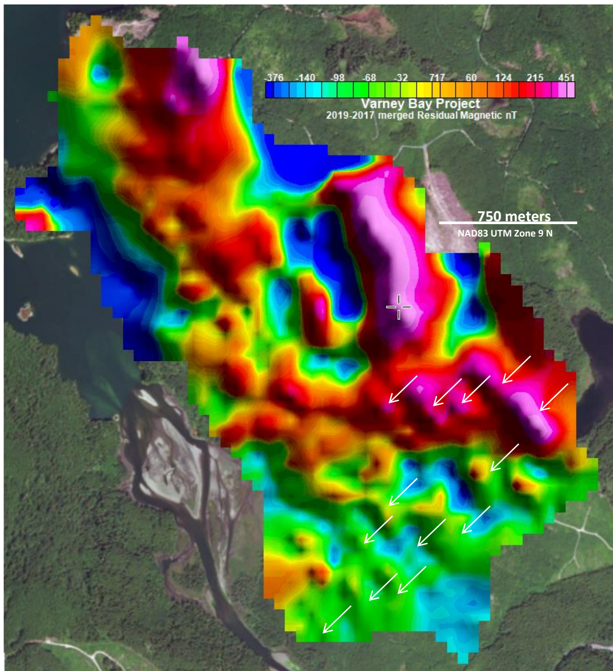
Figure 7. The 2019-2017 merged sun shaded IGRF corrected residual TMI image on Landsat. The raw data range is 4316 nT, the 60 m cell gridded range is 3284 nT. The arrows point out more-subtle line level offsets remaining in the residual magnetic data that require leveling.
