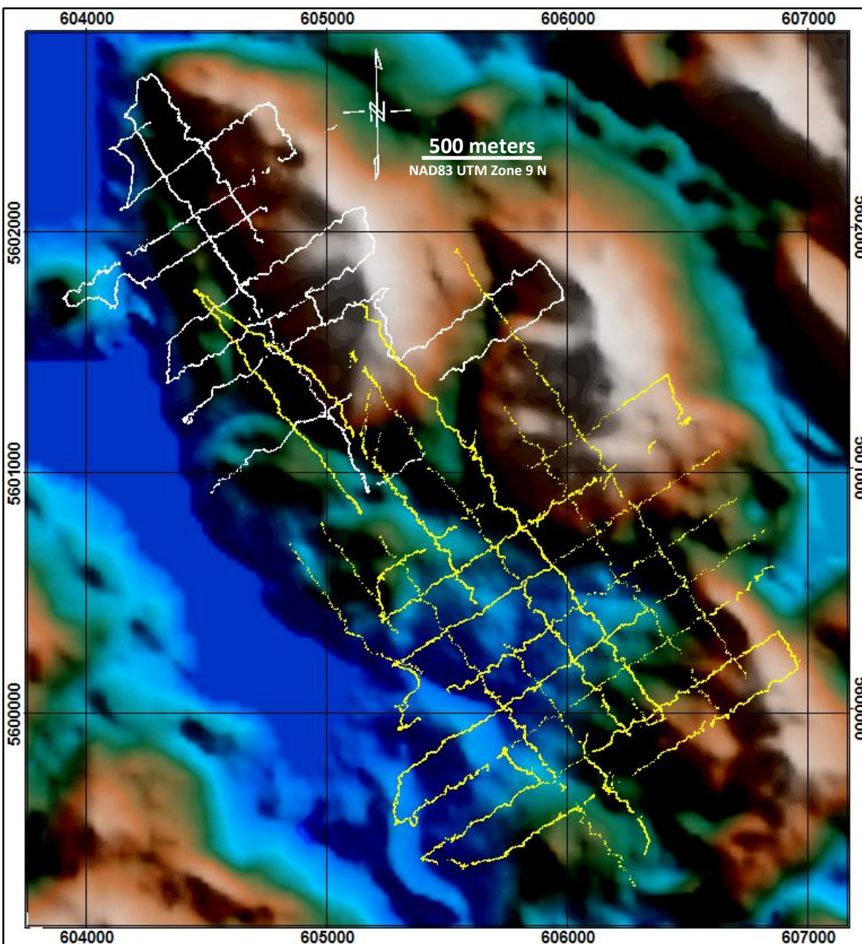
Figure 2. Varney Bay area SRTM image with the 2019 magnetic survey sample lines the white traces, 2017-2018 survey lines the yellow traces. There is 193 metres of topographic relief in the survey area.
