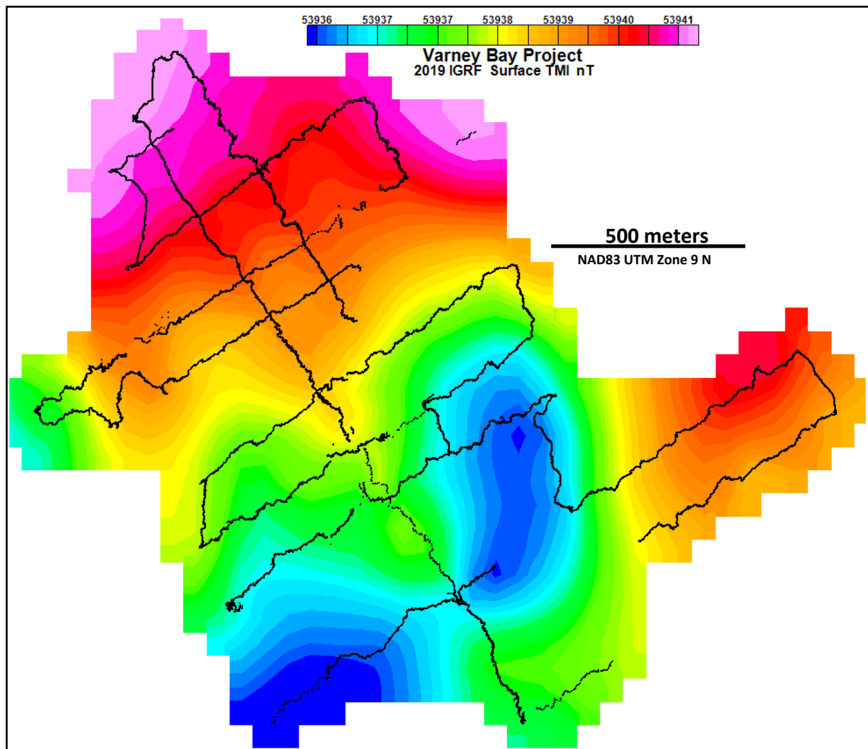
Figure 3. IGRF correction values across the 2019 Varney Bay grid, range is 7 nT.
