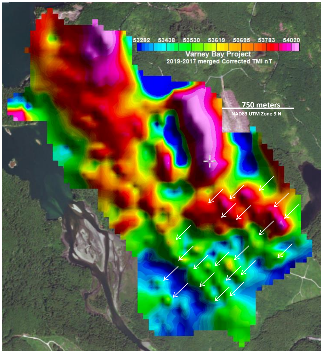
Figure 6. The 2019-2017 merged sun shaded base corrected TMI image on Landsat. The raw data range is 4588 nT, the 60 m cell gridded range is 3286 nT. There are obvious line level artifacts in the data as pointed out by the arrows; the 2017 data has higher background amplitude than the 2018 and 2019 data. The gradient shading exacerbates the line effects.
