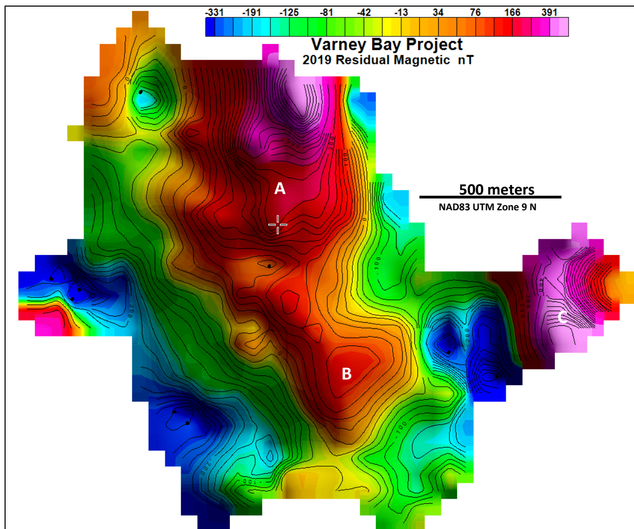
Figure 5. The sun shaded IGRF corrected residual magnetic image. The raw data range is 3595 nT, the 60 m cell gridded range is 1520 nT.
