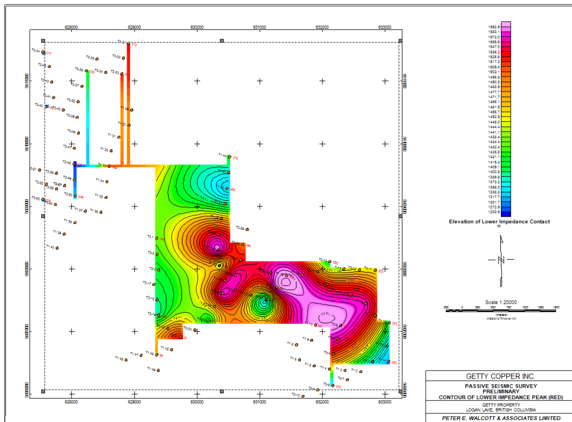
Modelled Elevation of lower impedance peak.
