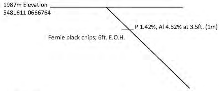
Figure 32 Drill Hole B-19-13
