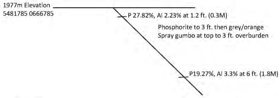
Figure 22 Drill Hole B-19-03
