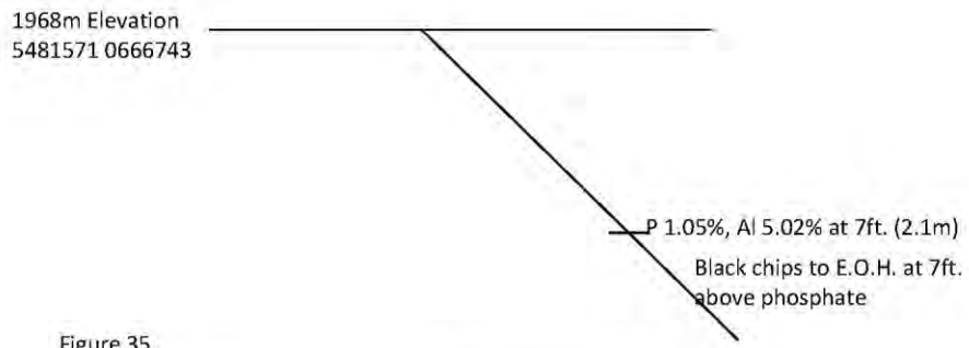
Figure 35 Drill Hole B-19-16
