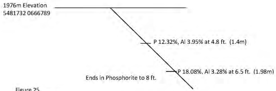
Figure 25 Drill Hole B-19-06
