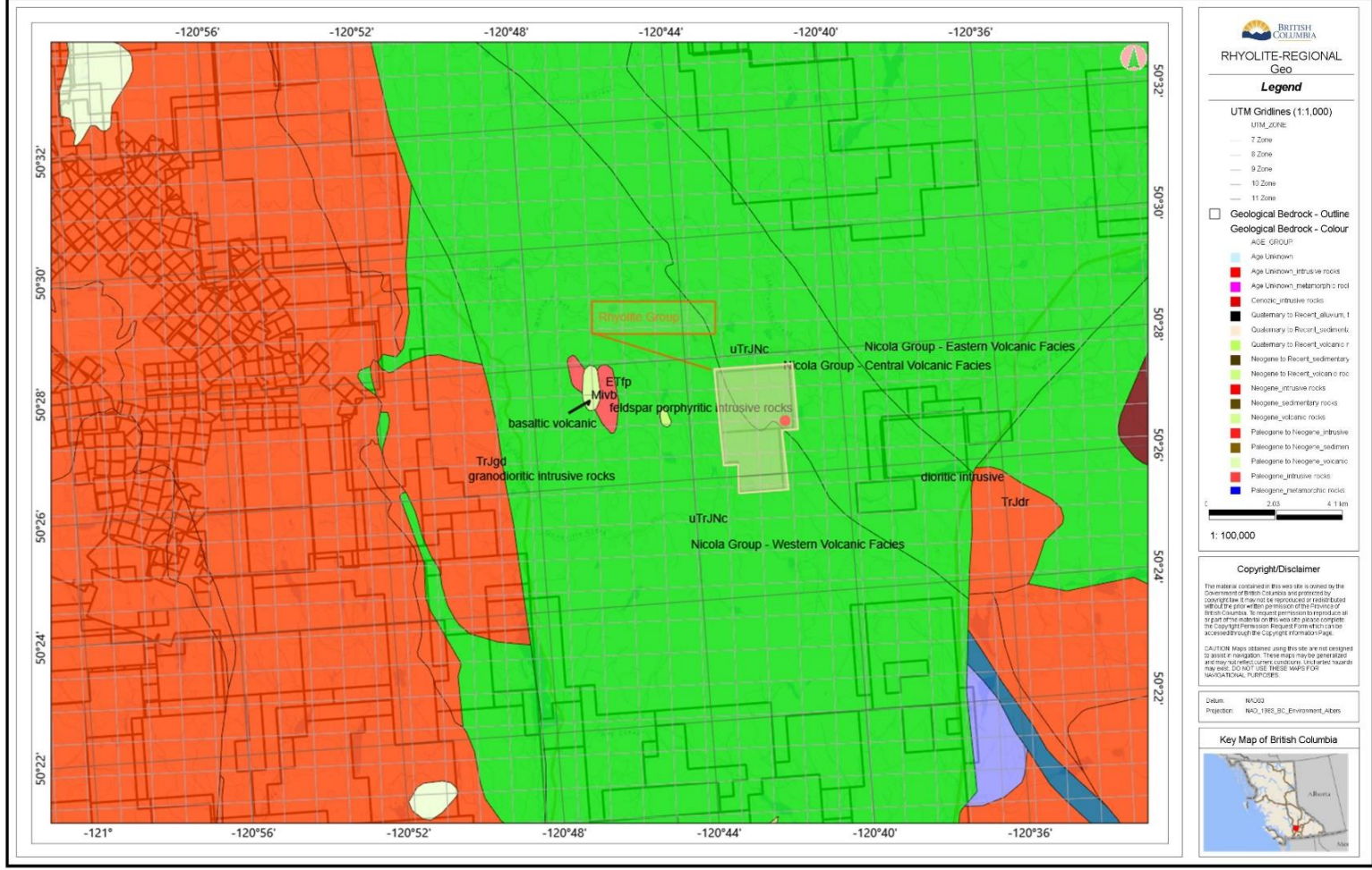
Figure 7 RHYOLITE CLAIM GROUP Regional Geology
