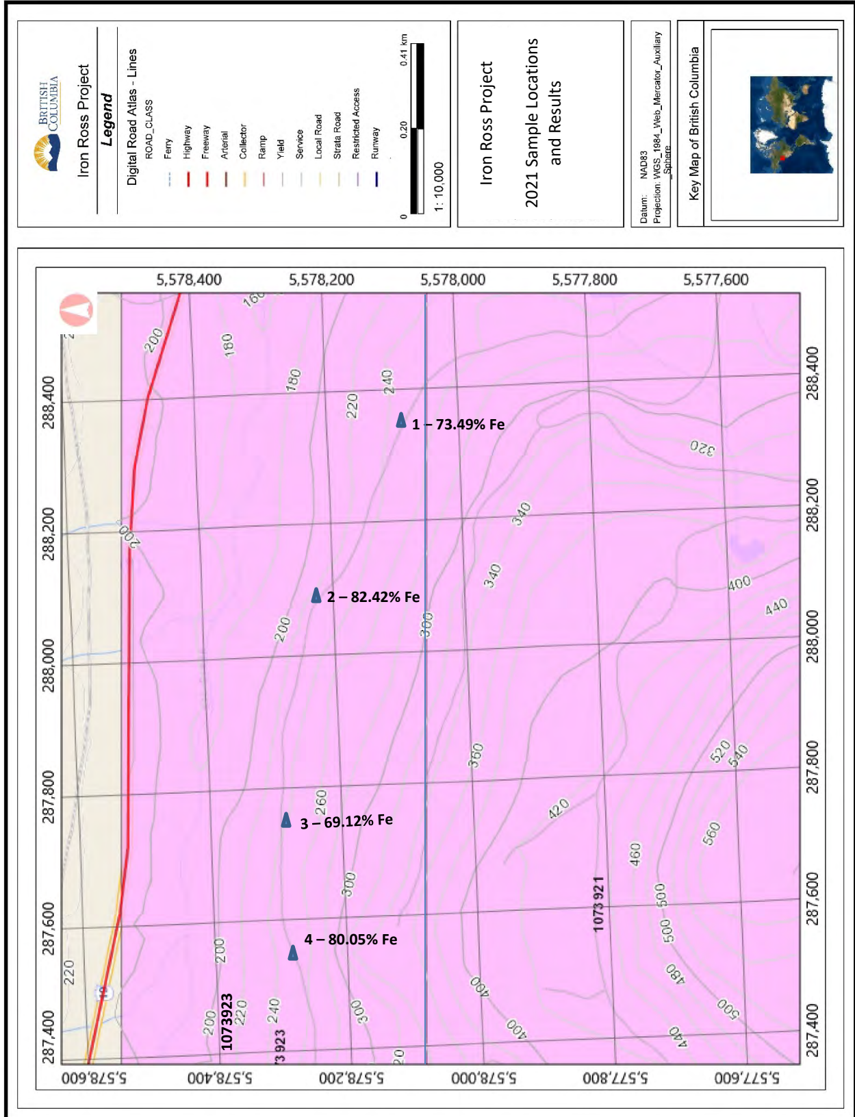
Figure 22 2021 Sample Locations and Results
