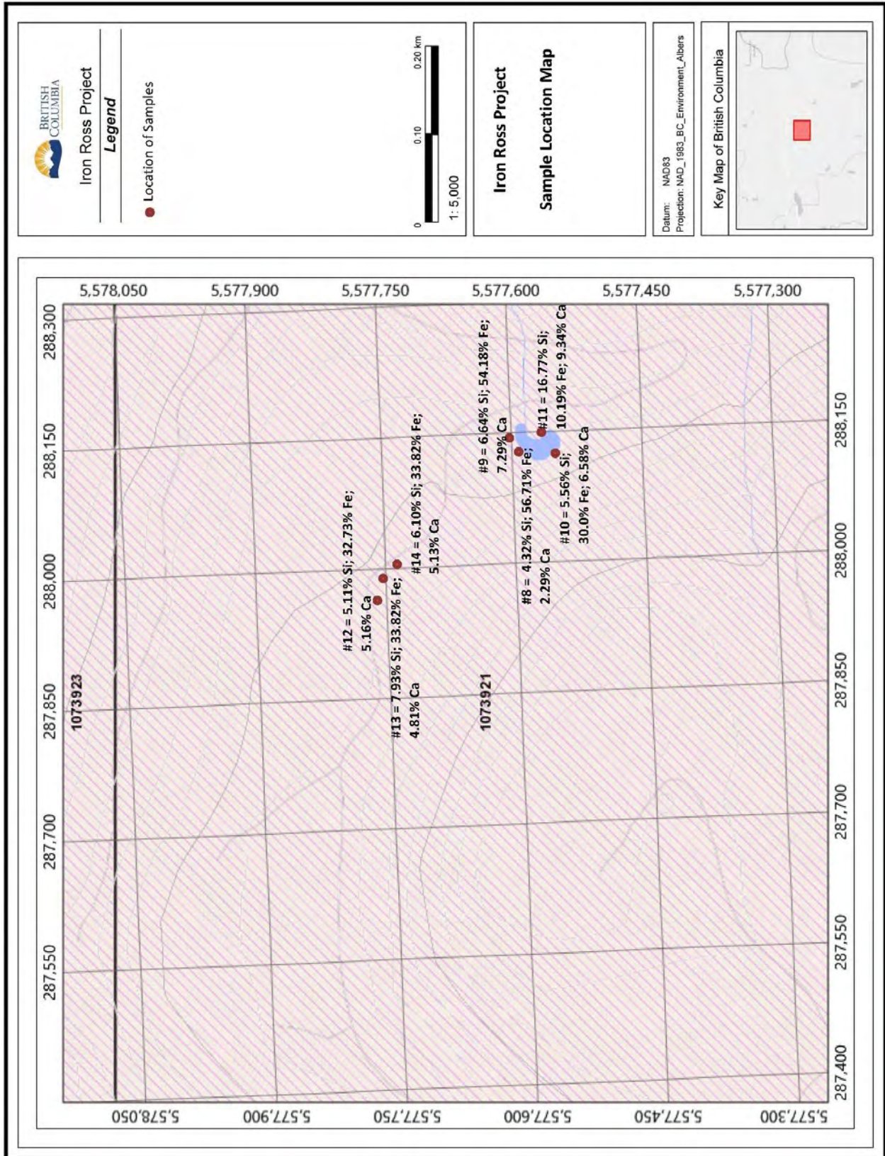
Figure 17 2020 Sample Location Map
