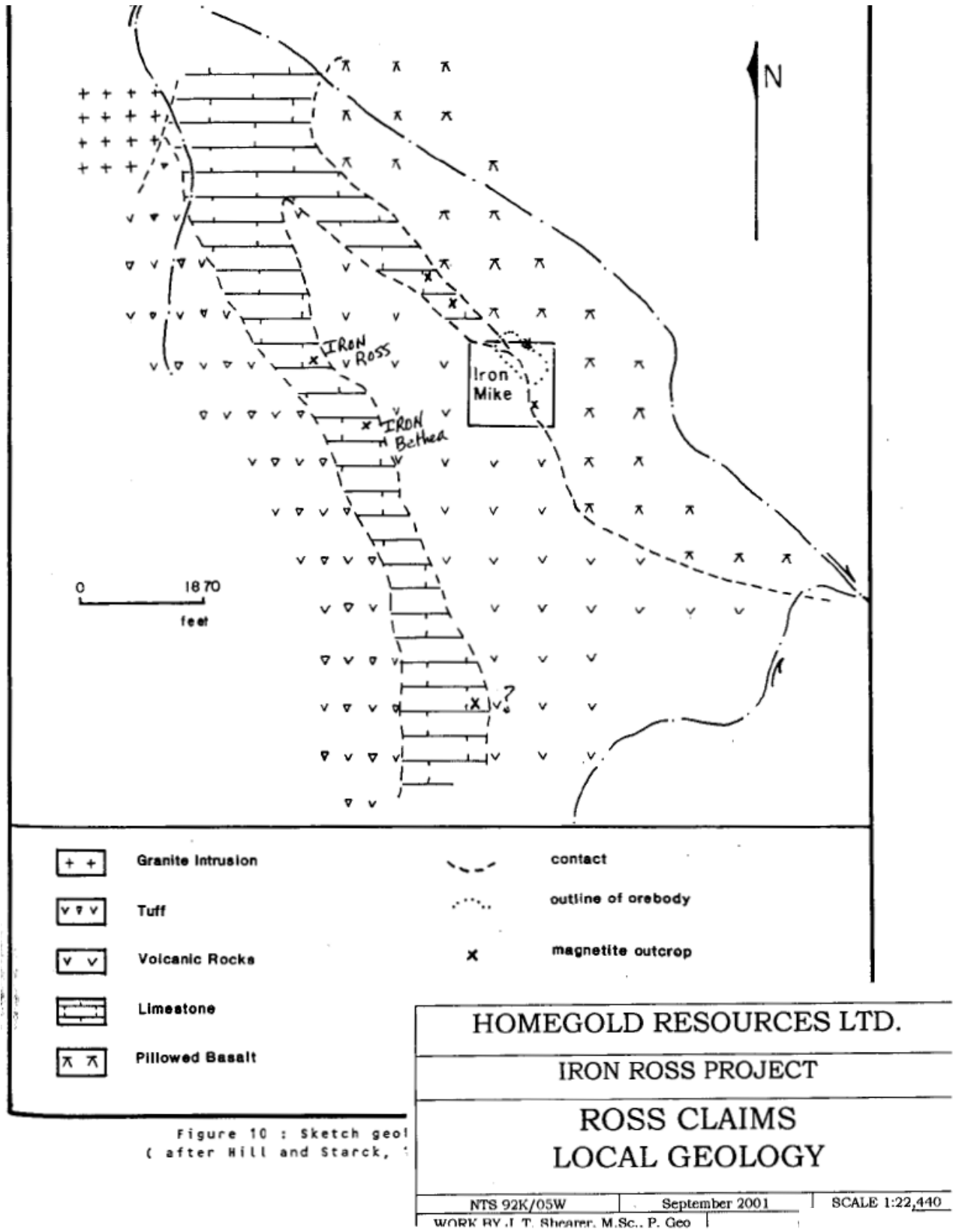
Figure 20 Local Geology (Generalized)
